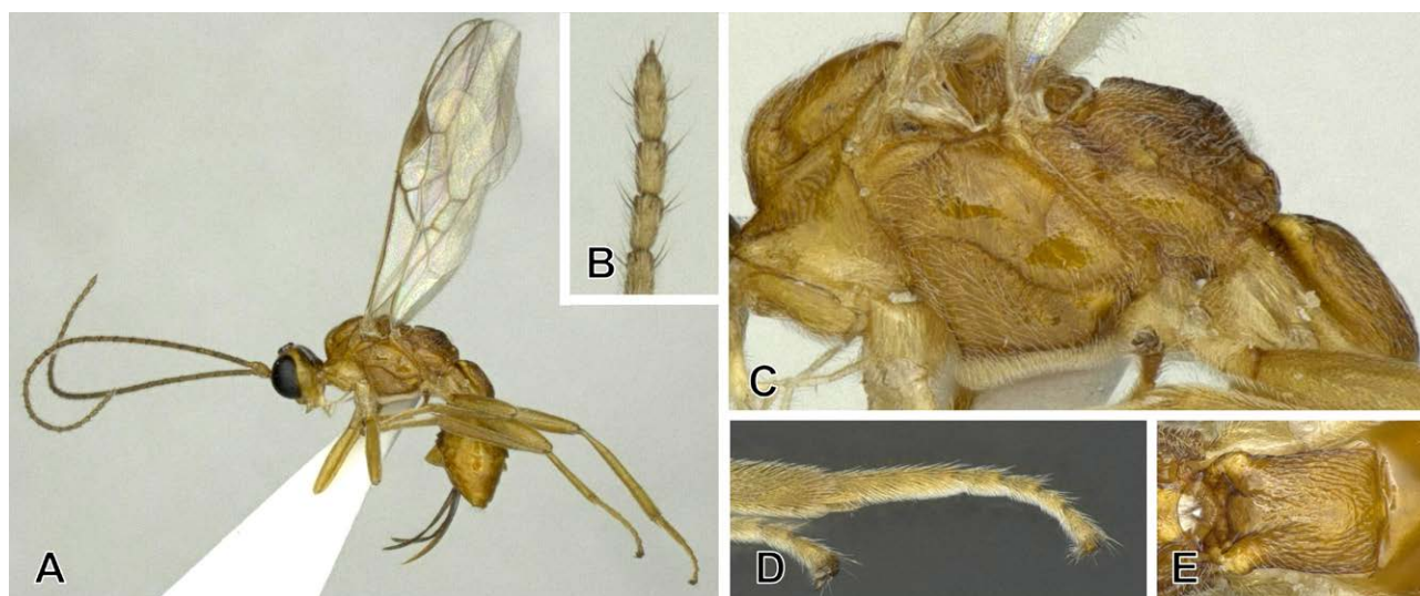
Fig. 23. Pygostolus falcatus (Nees), female, from Hyôgo Prefecture. — A, Habitus, lateral view; B, apical antennal segments; C, mesosoma and first metasomal tergite, lateral view; D, hind tarsus; E, first metasomal tergite, dorsal view.
