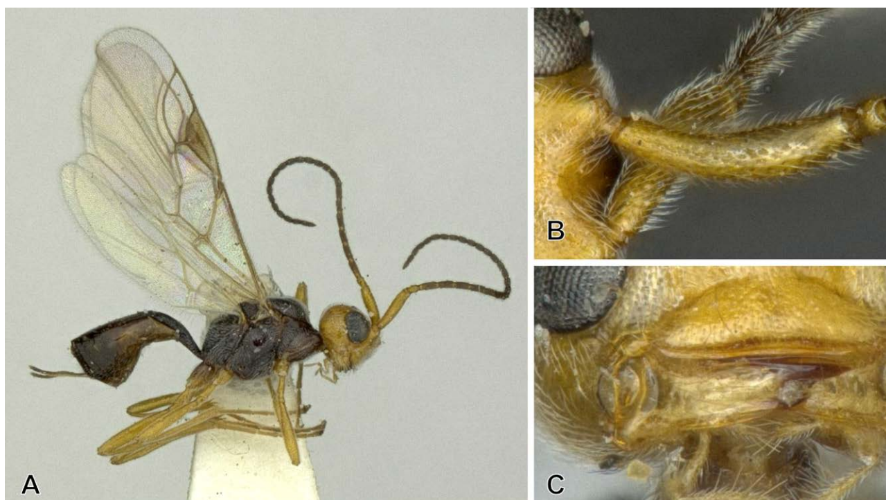
Fig. 26. Streblocera (Cosmophoridia) flaviceps (Marshall), female, from Tōkyō Prefecture. — A, Habitus, lateral view; B, scape, ventral view; C, head, ventro-frontal view.
