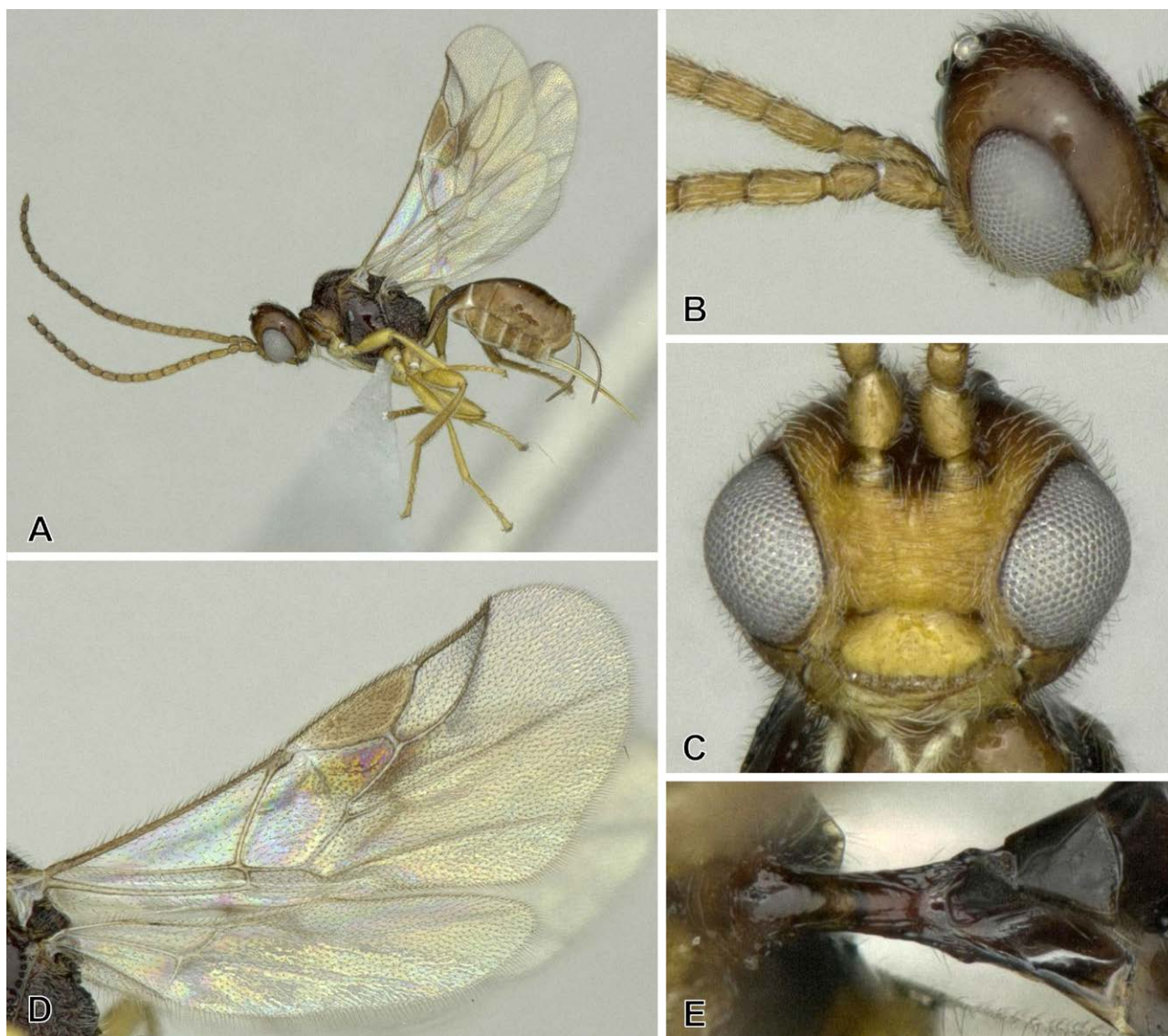
Fig. 30. Townesilitus deceptor (Wesmael), female, from Aichi Prefecture. — A, Habitus, lateral view; B, head, lateral view; C, head, frontal; D, wings; E, First metasomal tergite, ventral view.
