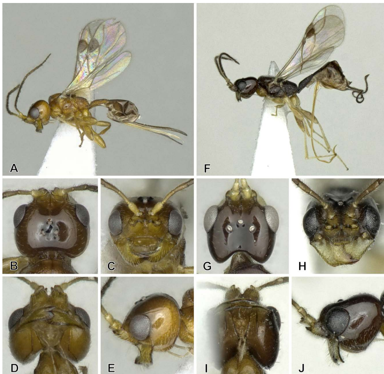
Fig. 7. Cosmophorus ( Cosmophorus ) sp., female, from Ōsaka Prefecture (A–E); C. (Eucosmophorus) sp., female, from Ishigaki Is. (F, H, I, J), and from Ishikawa Prefecture (G). — A, F, Habitus, lateral view; B, G, head, dorsal view; C, H, head, frontal view; D, I, Head, ventral view; E, J, head, lateral view.
