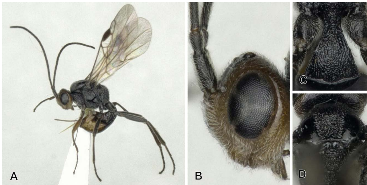
Fig. 9. Dinocampus coccinellae (Schränk), ♀, from Hokkaidō Prefecture. — A, Habitus, lateral view; B, head, lateral view; C, mesonotum, dorsal view, D, first metasomal tergite, dorsal view.
