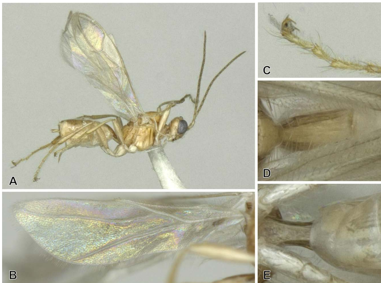
Fig. 28. Syntretus (Exosyntretus) elabsus (Papp), female, from Hokkaidô. — A, Habitus, lateral view; B, hind wing; C, hind claw; D, first metasomal tergite, dorsal view; E, same, ventral view.
