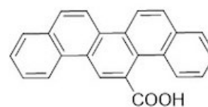
[5]phenacene-13-carboxylic acid
