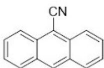
9-cyanoanthracene
