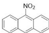
9-nitroanthracene
