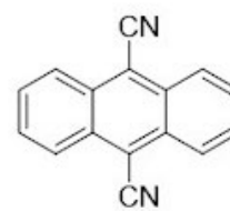
9,10-dicyanoanthracene
