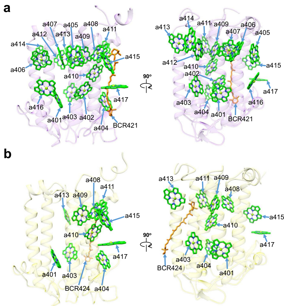
Fig. 3 | Structures of IsiA1-5 and IsiA1-4. Structures of IsiA1-5 (a) and IsiA1-4 (b) depicted in transparent cartoon model and arrangements of Chl and β-carotene
