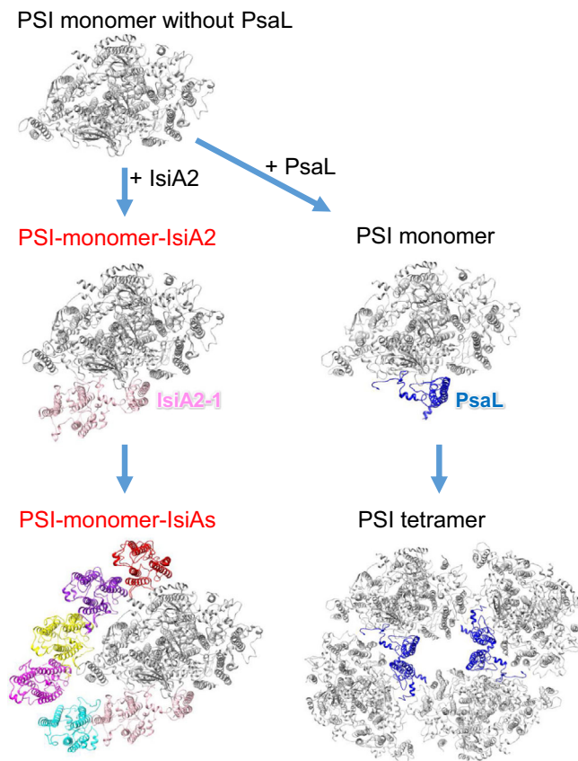
Fig. 8 | An assembly model proposed for the Anabaena PSI-IsiA supercomplex. The structures are viewed from the cytosolic side. The PSI monomer and tetramer structures are taken from 6JEO (PDB ID).
