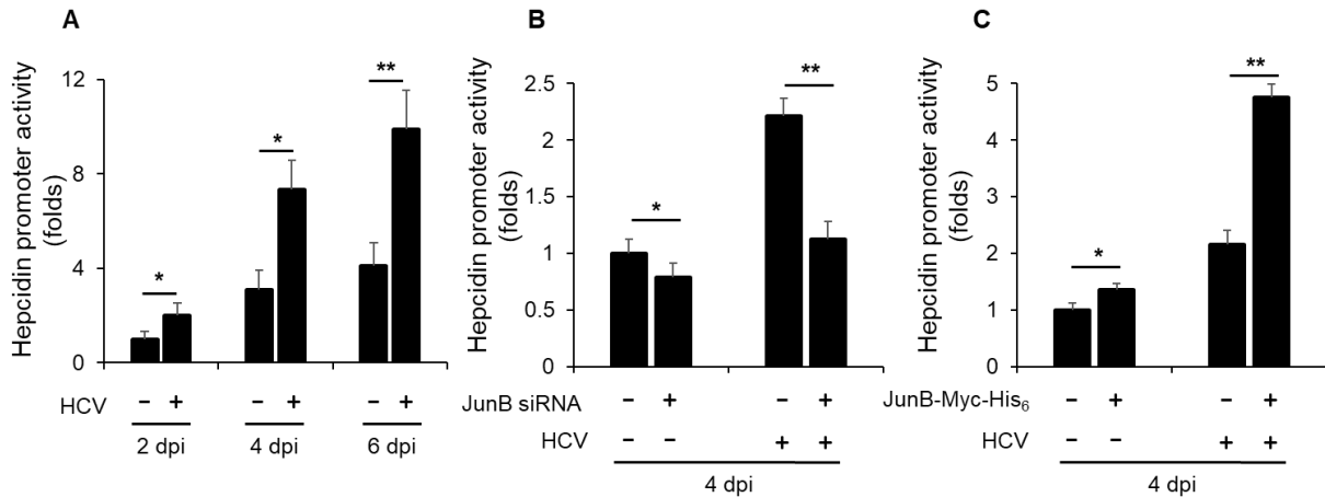
Fig. 5. JunB is involved in HCV-induced enhancement of hepcidin promoter activity.
