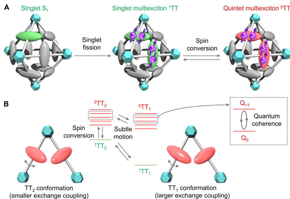
Fig. 1. Quintet multiexciton generation and its quantum coherence in an MOF. (A) SF followed by spin evolution via modulation of exchange interactions results in the formation of quintet multiexciton ^5\text{TT} in an MOF. (B) Suppressed chromophore motion in an MOF enables not only the spin conversion from ^1\text{TT} to ^5\text{TT} but also the quantum coherence of ^5\text{TT} over hundred nanoseconds even at room temperature.
