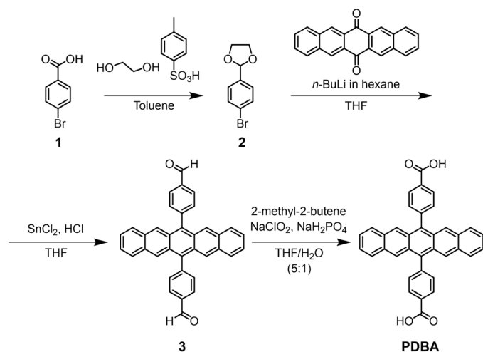
Fig. 7. Synthetic route of PDBA.
