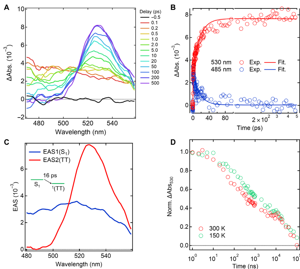
Fig. 3. TAS measurements of Pn-MOF. (A) Experimentally observed spectral evolution of the femtosecond TAS (excitation wavelength, 600 nm) of Pn-MOF in paraffin. (B) Temporal change of transient absorption at selected wavelengths and fitting curves from global analysis. (C) EAS obtained from global analysis based on the sequential model based on two components. EAS1 and EAS2 indicate the first and second components of EAS, respectively. (D) Temperature dependence of the transient absorption at 530 nm of Pn-MOF.
