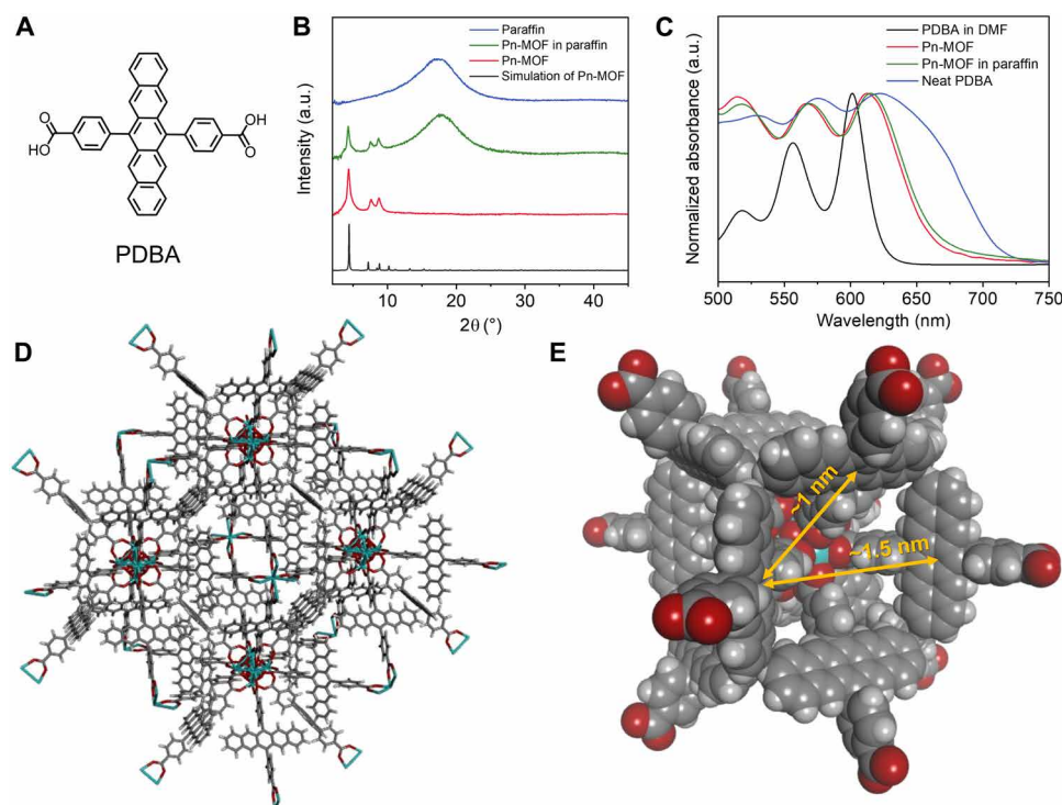
Fig. 2. Characterizations of Pn-MOF. (A) Chemical structure of PDBA. (B) Simulated PXRD pattern of Pn-MOF (black line) and experimental PXRD patterns of Pn-MOF (red line), Pn-MOF in paraffin (green line), and paraffin (blue line). a.u., arbitrary units. (C) UV-vis absorption spectra of 1 mM PDBA in DMF (black line), Pn-MOF (red line), neat PDBA solid (blue line), and Pn-MOF in paraffin (green line). (D) Simulated structure of Pn-MOF with UiO-68-type topology. (E) The nearest and second nearest pentacene moieties in Pn-MOF.
