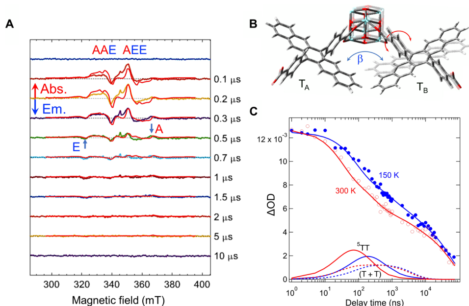
Fig. 4. Transient EPR spectra of Pn-MOF. (A) TREPR spectra for different delay times of Pn-MOF in paraffin at room temperature. Spectrum simulations by the rotation model analysis in Fig. 5 are shown by the red lines. (B) Conformations of the quintet TT_1 and TT_2 . The blue arrow represents dihedral angle ( \beta ) of the aromatic plane in T_B relative to T_A in the T_A T_B pair. (C) Decay profiles of the absorbance changes in nanosecond TAS ( \Delta OD ) by the multiexcitons at temperatures of 300 K (red circles) and 150 K (blue circles), together with simulated profiles by the rotation model analysis (red and blue lines). Contributions of {}^5TT and SCTP ( T + T ) are shown by the solid and dashed lines, respectively, at 300 K (red line) and 150 K (blue line).
