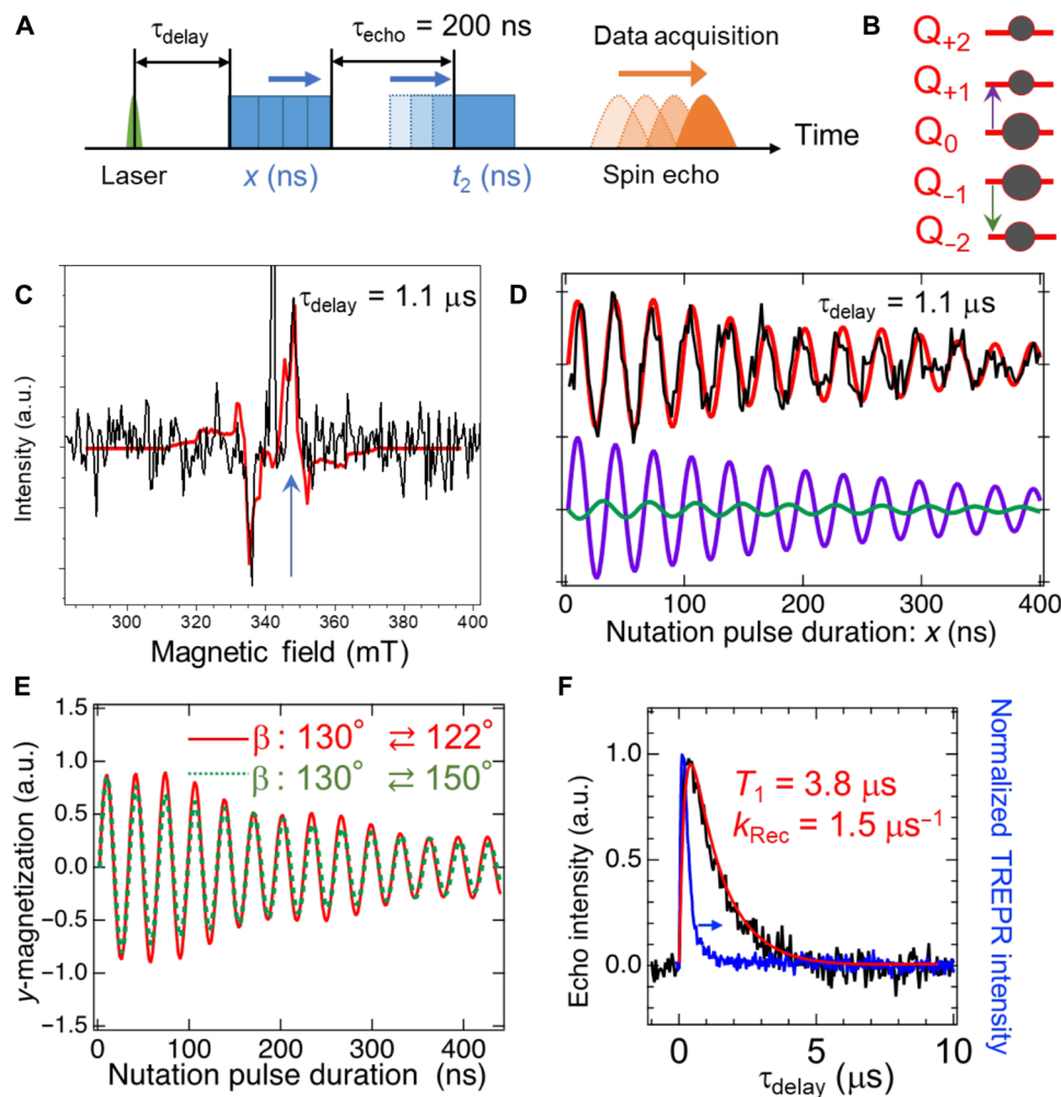
Fig. 6. Transient nutation of the quintet state at room temperature. (A) Pulse sequence of the transient nutation measurement. (B) Two main quantum gates detected by the pulsed microwave at B_0 = 348.1 mT in the quintet sublevels. (C) Echo-detected EPR spectrum at \tau_{\text{delay}} = 1.1 \mu\text{s} . The durations of the first and second pulses are x = 8 ns and t_2 = 16 ns, respectively. Fitting result using eq. S15 and table S5 is shown as a red line. (D) Transient nutation profiles as a function of x in (A) at \tau_{\text{delay}} = 1.1 \mu\text{s} using t_2 = 16 ns. The simulated profile is shown by a red line considering the anisotropic sublevel populations. At the bottom, decomposition of the computed nutation data by the gates Q_{0,\pm 1} and Q_{\pm 2,\pm 1} are shown by purple and green lines, respectively. (E) Simulated profiles by the different rotation models. The red solid line corresponding to the red line in (D) is computed by the conformation motion between the dihedral angles of \beta = 130^\circ and 122^\circ of the T_A T_B pair for TT_1 and TT_2 , respectively. Green dashed line is obtained with considering the large dihedral angle change between \beta = 130^\circ and 150^\circ in Fig. 4B. (F) Dependence of \tau_{\text{delay}} on the echo intensity (black line) employing x = 8 ns, t_2 = 16 ns, and \tau_{\text{echo}} = 200 ns with B_1 = 0.45 mT together with delay time dependence of the CW-TREPR intensity at 351 mT in Fig. 4A (blue line). Fitting result using eq. S1 and table S5 is shown as a red line.
