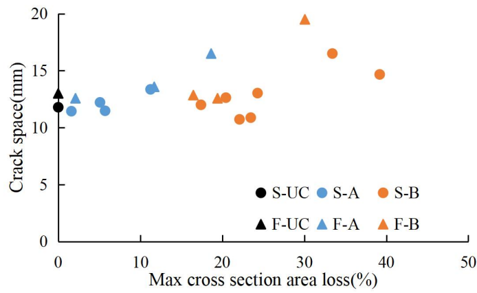
Fig. 5.9 Crack space
