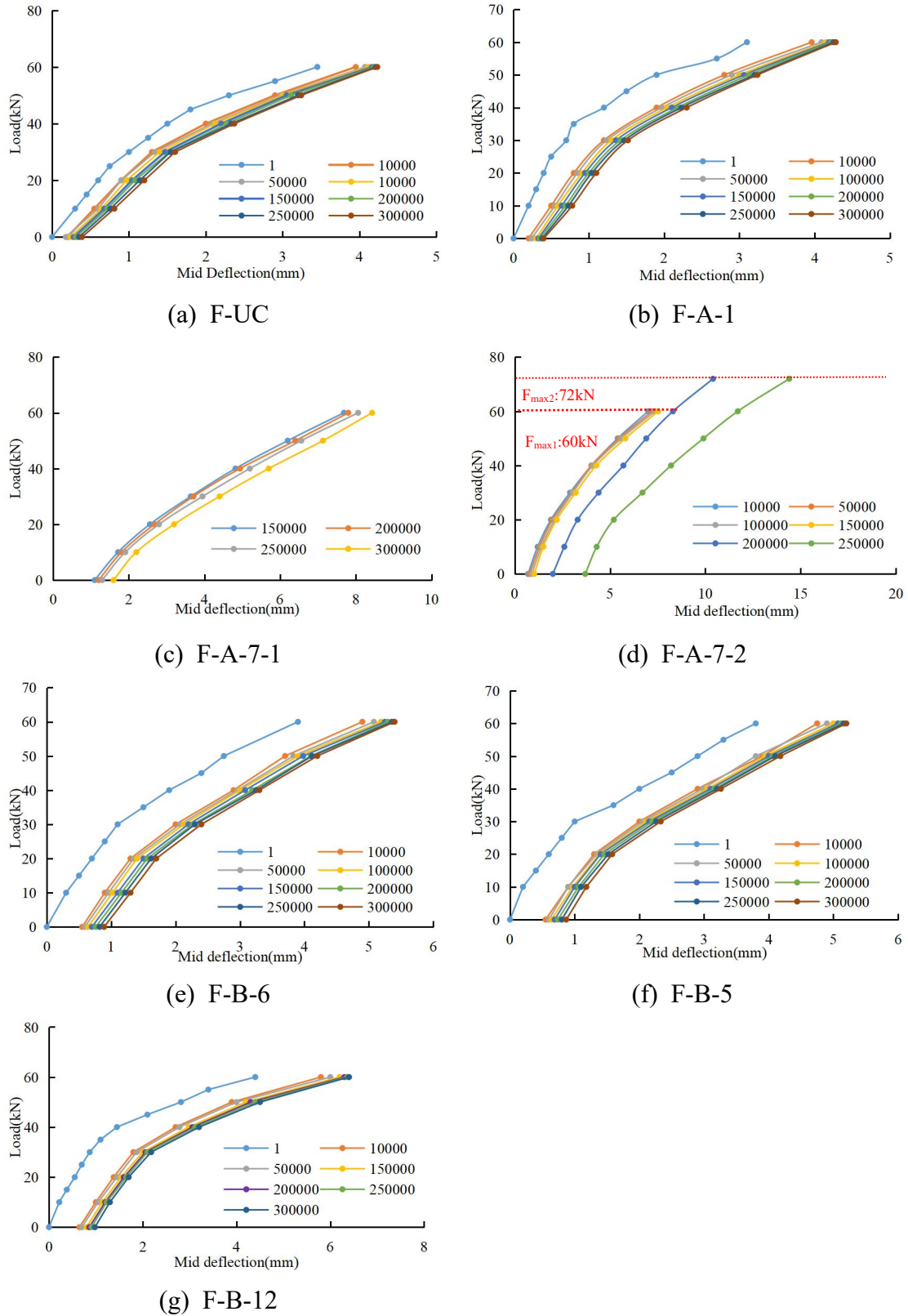
Fig 5.6 Load- deflection curve
