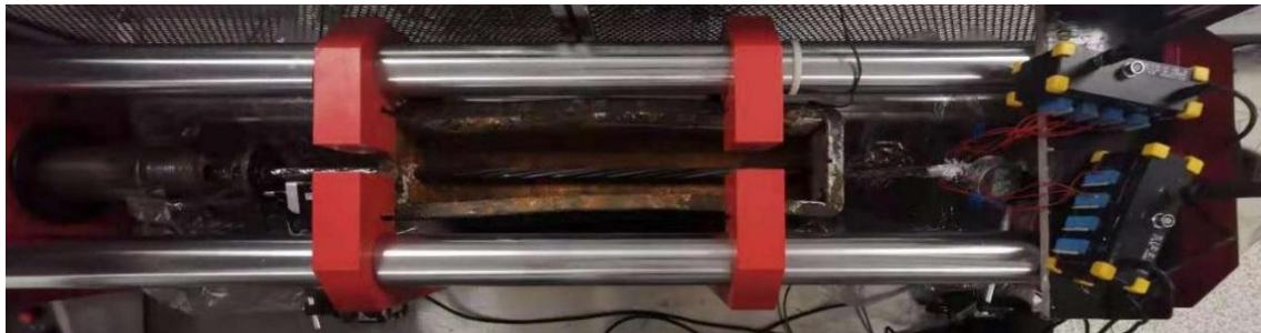
Fig. 2.2 Corrosion test setup with a relaxation test machine
