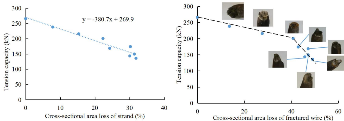
(a) Cross-sectional area loss of PC strand (b) Cross-sectional area loss of fractured wire
