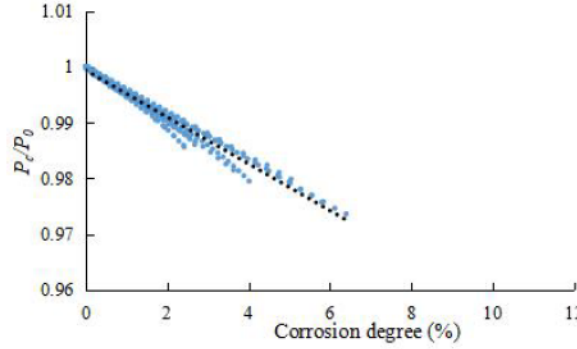
Fig.2.16 Relationship between prestressing force and corrosion degree
