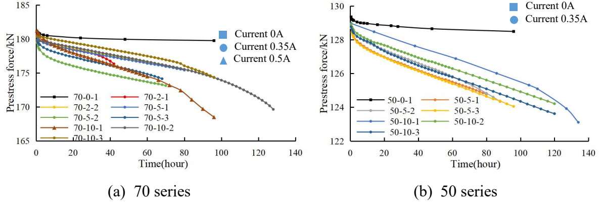
Fig. 2.8 Prestressing force versus corrosion time curve
