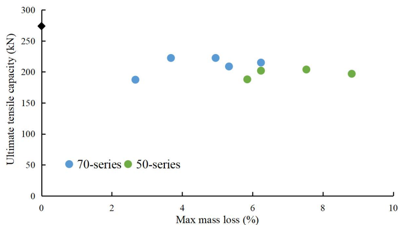
Fig. 2.19 Relationship between ultimate tensile capacity and corrosion degree (Max mass loss)
