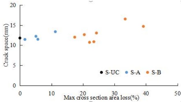
Fig. 4.10 Crack space versus max cross section area loss(%)
