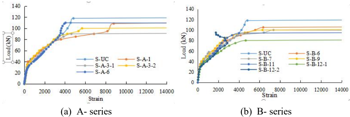
Fig. 4.11 Strain of longitudinal steel bars versus load
