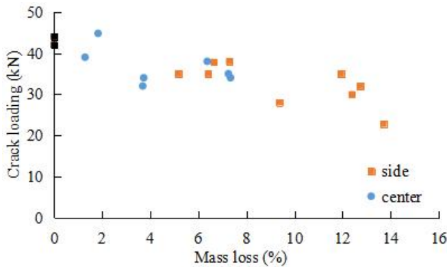
Fig. 3.10 Crack load versus mass loss of strand
