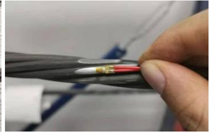
Fig. 2.23 Pasted strain gauge
