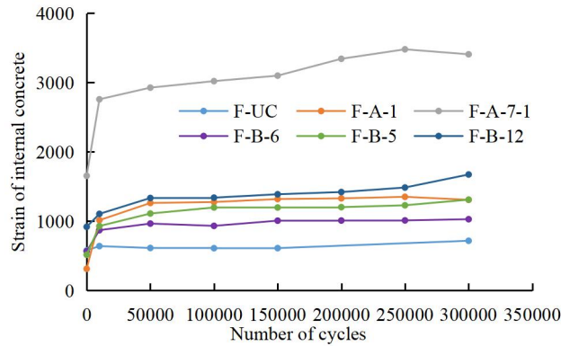
Fig. 5.14 Strain of internal concrete versus number of cycles
