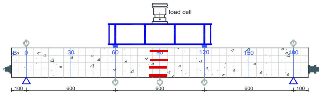
Fig. 4.1 Loading diaram
