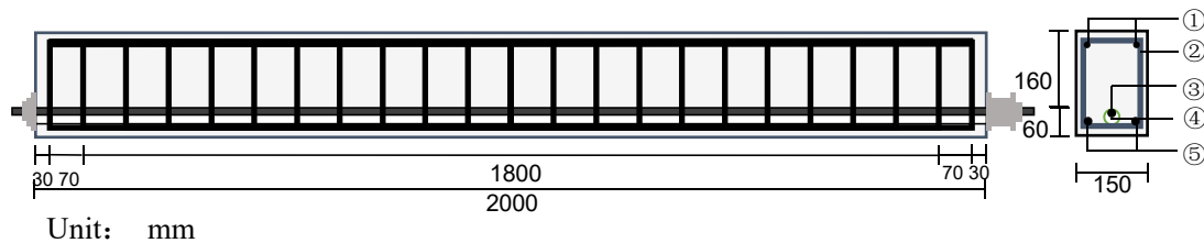
Fig. 3.1 Beam detail
