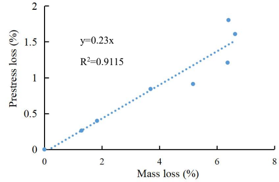
Fig. 3.12 Prestress loss in first stage
