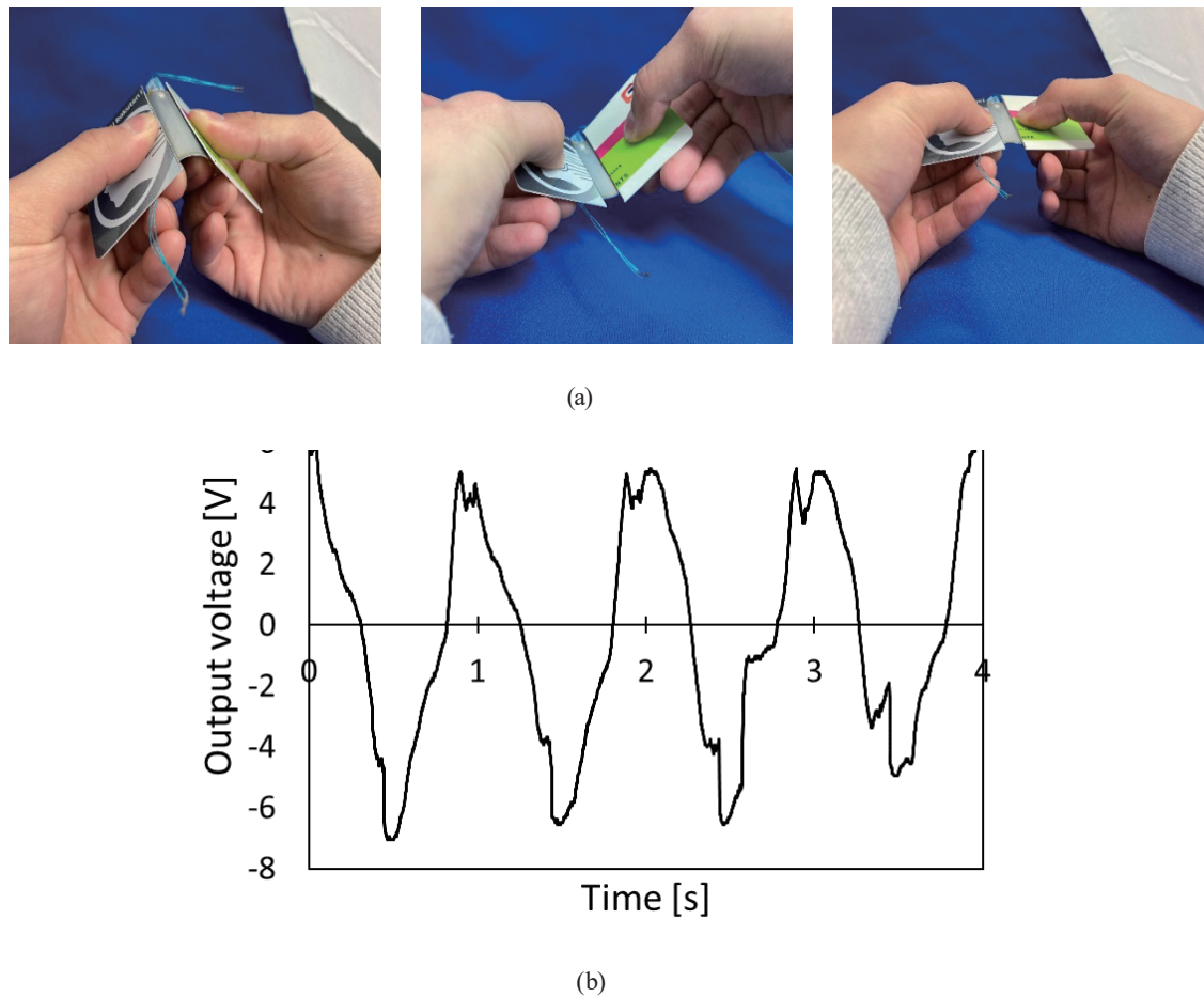
Fig. 5. (Color online) Manual bending operation during output power measurement of card-type PEH. (a) Pictures of bending operation and (b) output voltage.
