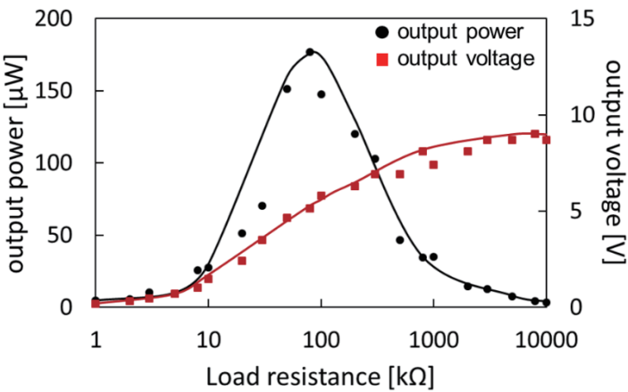
Fig. 6. (Color online) Output voltage and output power of PEH as a function of load resistance.
