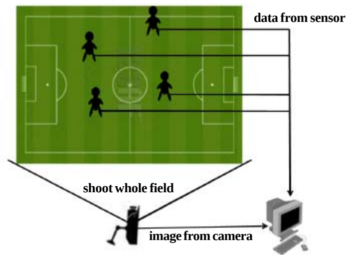
Figure 1. System architecture
