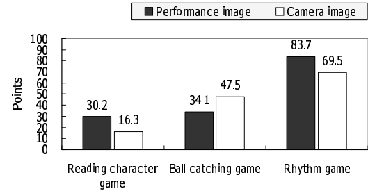
Fig. 18. Game scores
