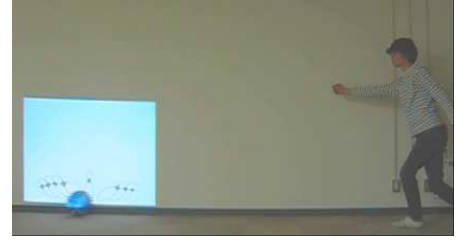
Fig. 24. Bowling performance
