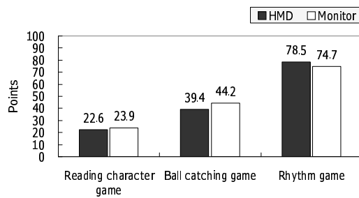
Fig. 18. Game scores
