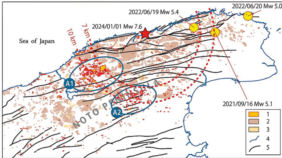
Fig. 6 Synthesis map: The January 2024 co-seismic landslides are not controlled by past- and active landslides.
