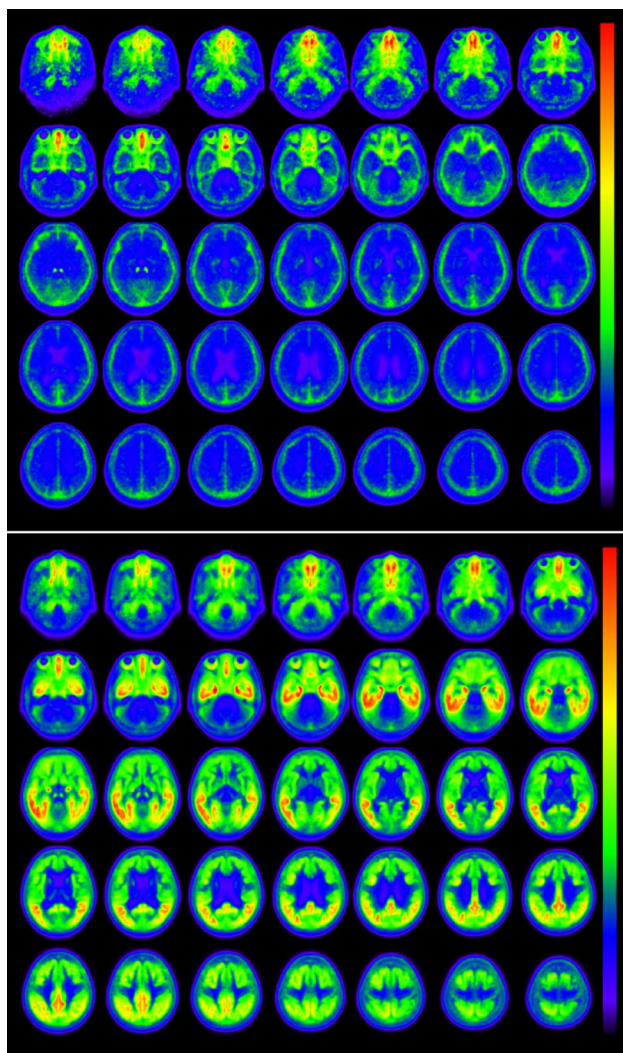
Fig. 3 Mean ^{18}\text{F} -MK-6240 images of the tau-negative and -positive subjects. A: Mean ^{18}\text{F} -MK-6240 images of the tau-negative subjects ( n=9 ). B: Mean ^{18}\text{F} -MK-6240 images of the tau-positive subjects ( n=26 )
