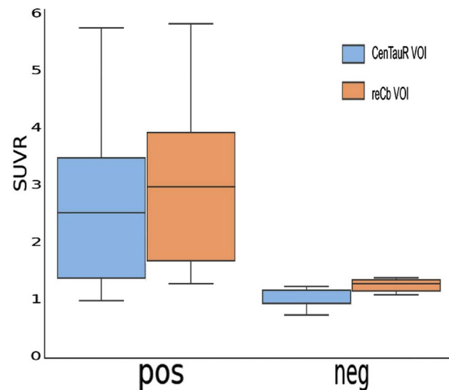
Fig. 5 Comparison of the SUVRs calculated using the restricted cerebellar VOI and CenTauR cerebellar VOI in the tau-negative and tau-positive groups
