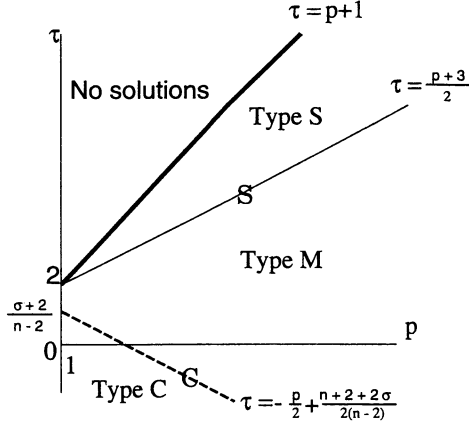
Fig. 4. Structure of solutions for (3.5) with \sigma \leq 2(n - 3) .
