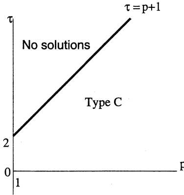
Fig. 2. Structure of solutions for (3.3) with \sigma \leq -2 .
