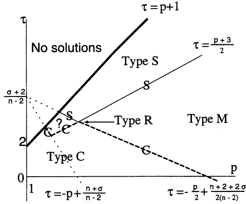
Fig. 5. Structure of solutions for (3.5) with \sigma > 2(n - 3) .
