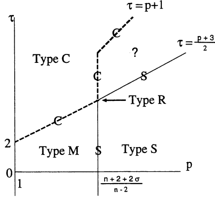
Fig. 1. Structure of solutions for (3.1) with \sigma > -2 .
