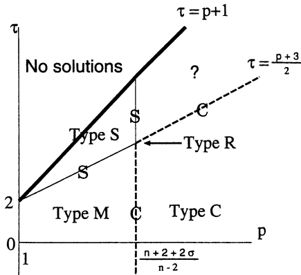
Fig. 3. Structure of solutions for (3.3) with \sigma > -2 .
