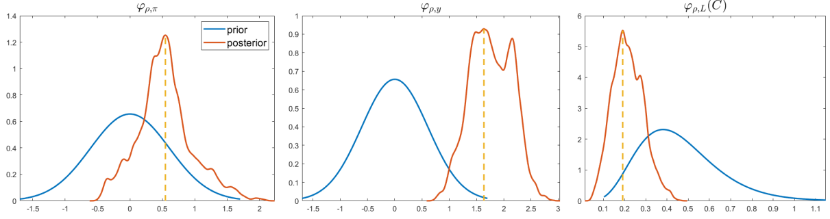
Figure B3: Prior and Posterior Distributions of the Feedback Coefficients of the RR-ratio Rule
