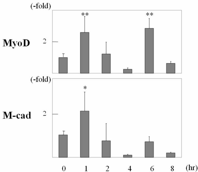
Figure 4. GH induced the bimodal expression of MyoD (upper panel) 1 h and 6 h after the stimulation by GH. On the other hand, GH increased M-cadherin expression 1 h but not 6 h after the stimulation by GH (lower panel). * p < 0.05 , ** p < 0.01 vs. time point 0 ( n = 5 in each group).
