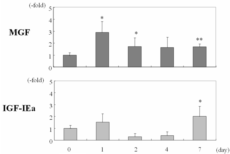
Figure 3. Chemical damage on the C2C12 cells induced the expressions of MGF (upper panel) and IGF-IEa (lower panel) on days 1 and 7, respectively, after treatment with bupivacaine. * p < 0.05 , ** p < 0.01 vs. time point 0 ( n = 5 in each group).
