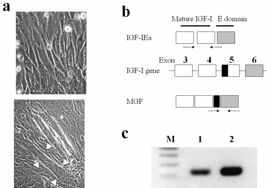
Figure 1. (a) Morphological changes in the C2C12 cells before and after differentiation from mononucleated myoblasts (upper panel) into mature myotubes (lower panel, arrowhead). (b) Schema of the mouse IGF-IEa and MGF cDNAs. The arrows indicate the position of specific primers for PCR amplification. (c) Detection of a specific band of IGF-IEa (lane 1) or MGF (lane 2) cDNA in the C2C12 cells. Products amplified by RT-PCR were separated on 2% agarose gel and visualized with ethidium bromide staining. M denotes the molecular weight marker.
