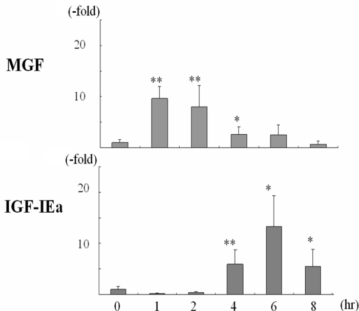
Figure 2. GH increased the expression of MGF and IGF-IEa in C2C12 cells. The mRNA levels of MGF (upper panel) and IGF-IEa (lower panel) was increased and the peak levels were reached at 1 h and 6 h, respectively, following stimulation by 100 ng/ml of GH. * p < 0.05 , ** p < 0.01 vs. time point 0 ( n = 5 in each group).
