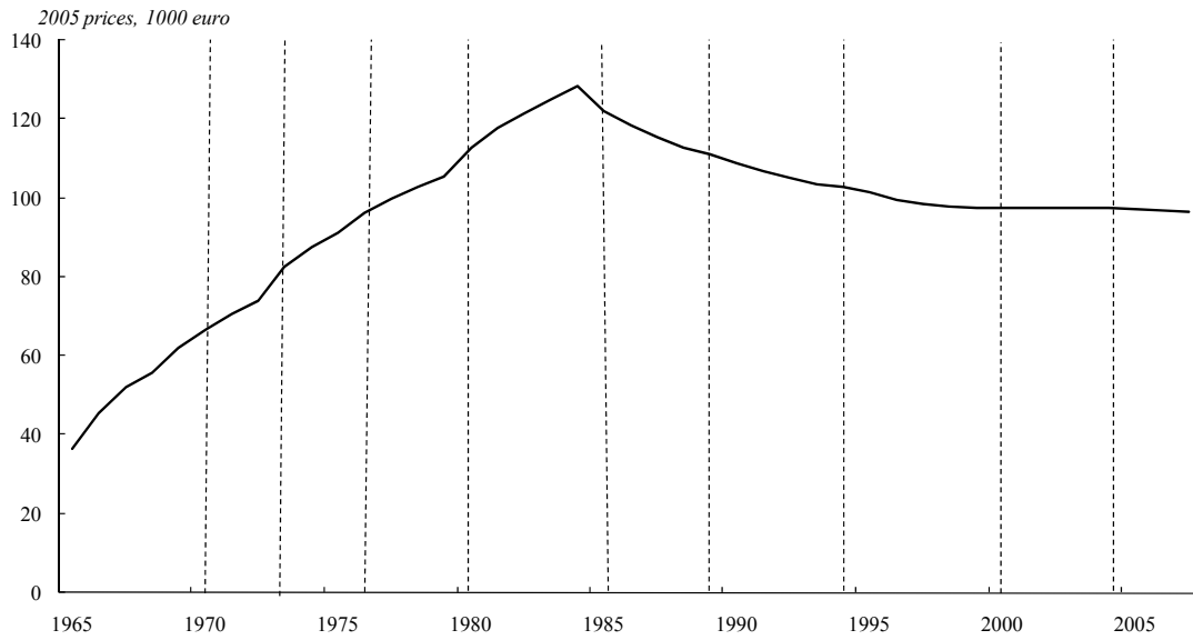
Figure 6. Annual average SSW (Wbar)
