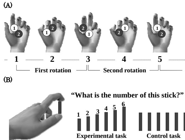
Figure 2. One run of the 2-ball rotation task performed using the left hand (A), and representative illustration of the perceptual learning task to improve the ability to discern the length of wooden sticks held between the left thumb and the left index finger (B). A: The participant rotates the 2 balls around each other on the palm in a counter-clockwise direction (phases 1–5). At the end of one rotation, the positions of the balls are exchanged. B: We used 6 wooden sticks of lengths 20, 22, 24, 26, 28, and 30 mm for perceptual learning. For the control task, the participants held a stick of the same length (25 mm) 6 times.
