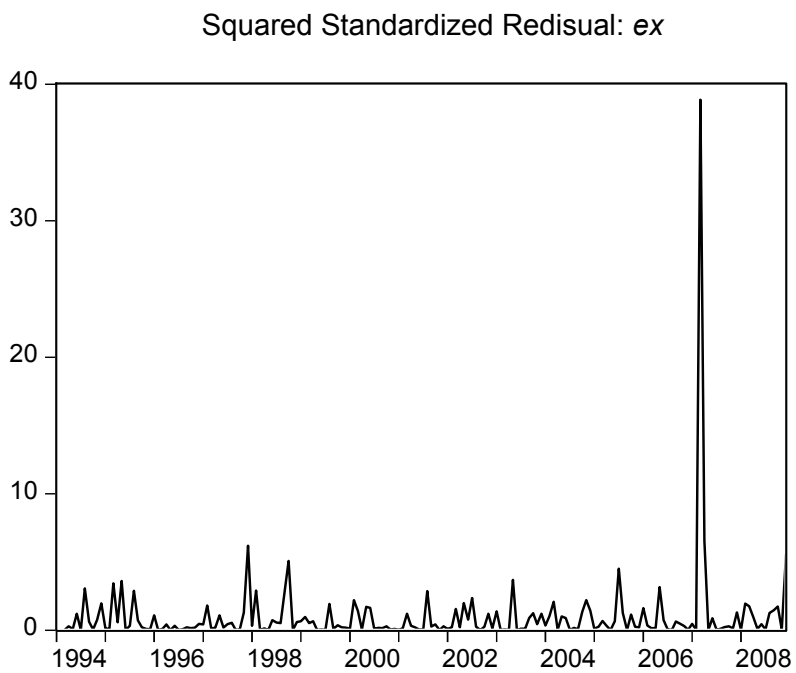
FIGURE 2. Squared Standardized Residuals
