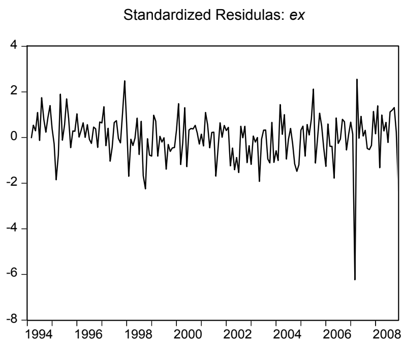
FIGURE 1. Standardized Residuals
