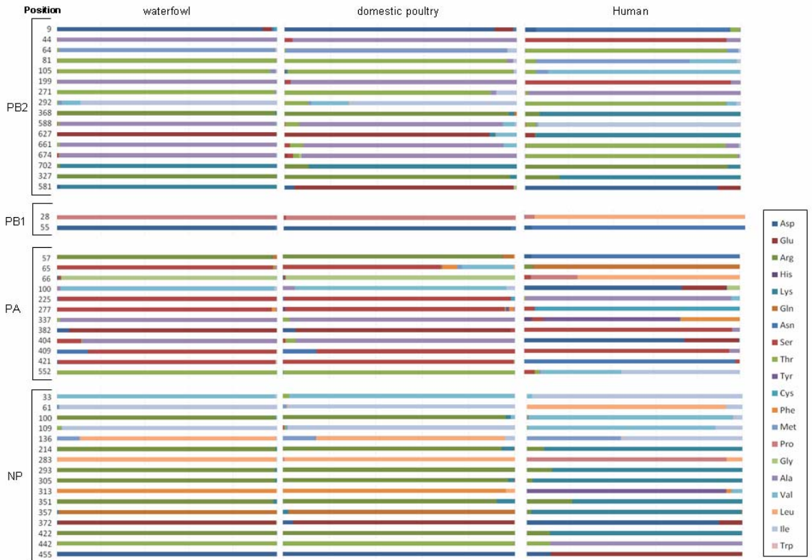
Figure 3. Conserved amino acids specific to species.
