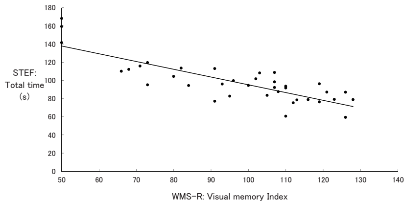
Figure 1: STEF total time and WMS-R visual memory index (n = 35: MCI)
