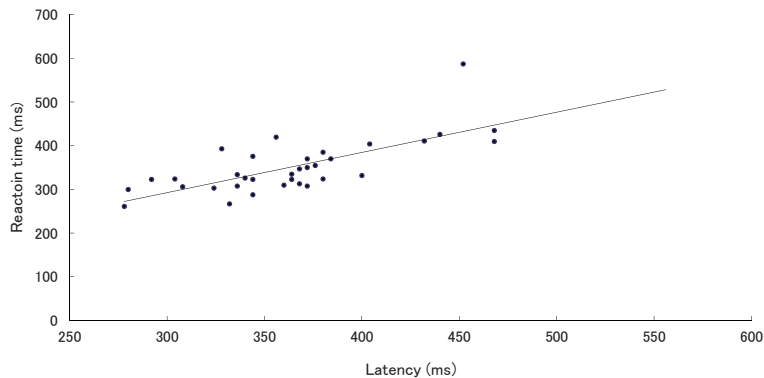
Figure 2: P300 latency and reaction time (n = 35: MCI)
