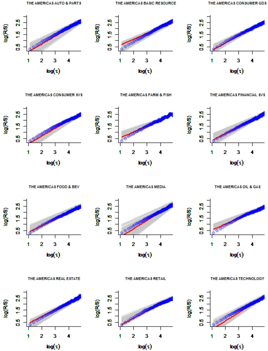
Figure 1: Bootstrapped regressions
