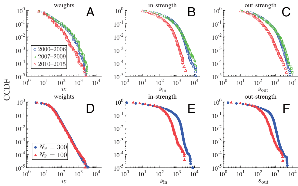
Fig. S3. CCDF of edge weights and strength. The in- and out-strength of bank i are defined as s_{\text{in},i} = \sum_{j \neq i} w_{ji} and s_{\text{out},i} = \sum_{j \neq i} w_{ij} , respectively. (A)–(C) The data. (D)–(F) The model.
