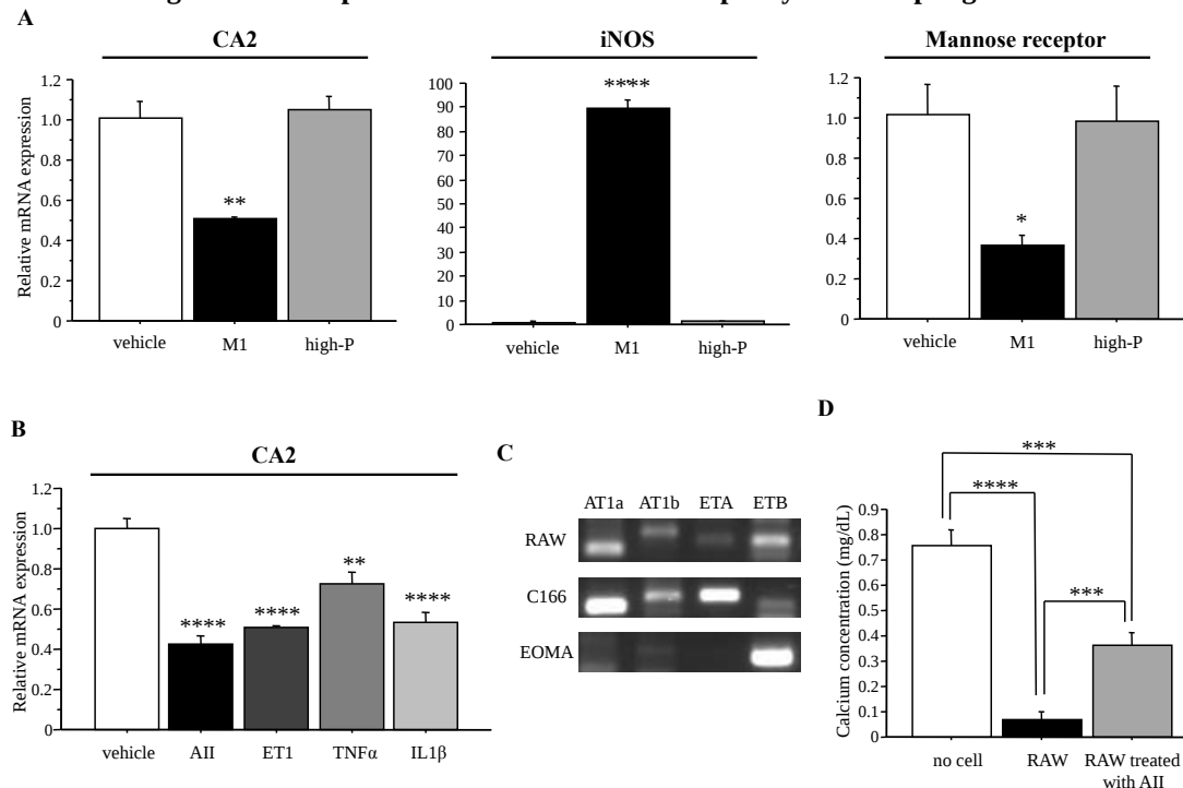
Figure 4. CA2 expression is regulated by various stimuli in macrophages.
