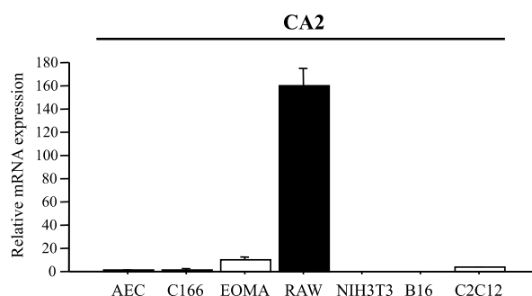
Figure 2. Expression of CA2 and V-ATPase in various types of cells. (A and B) Quantitative analysis for CA2 (A) or vacuolar H + -ATPase subunit c (B) mRNA expression in various cells. AEC, mouse aortic endothelial cells; C166, mouse endothelial cell line; EOMA, mouse endothelial cell line; RAW, mouse macrophage cell line; NIH3T3, mouse fibroblast cell line; B16, mouse melanoma cell line; C2C12, mouse myoblast cell line. Data are presented as mean \pm SE, n = 3 each.
