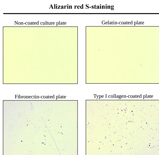
Figure 1. Establishment of cell free assay system for the analysis of ectopic calcification.
