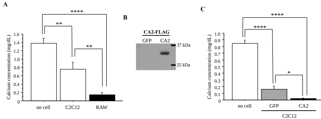
Figure 3. Macrophages effectively decalcify the ectopic calcification. (A) Quantification of remaining calcium precipitates in the calcification plates treated with no cell, C2C12 cells, or RAW cells. Data are presented as mean \pm SE, n = 11 for the plates with no cell; n = 10 each for the plates with cells. **P < 0.01 and ****P < 0.0001 . (B) Immunoblotting for CA2 tagged with FLAG in C2C12 cells transfected with either GFP or CA2 expression construct. (C) Quantification of remaining calcium precipitates in the calcification plates treated with no cell or C2C12 cells transfected with either GFP or CA2 expression construct. Data are presented as mean \pm SE, n = 6 each. *P < 0.05 and ****P < 0.0001 .
