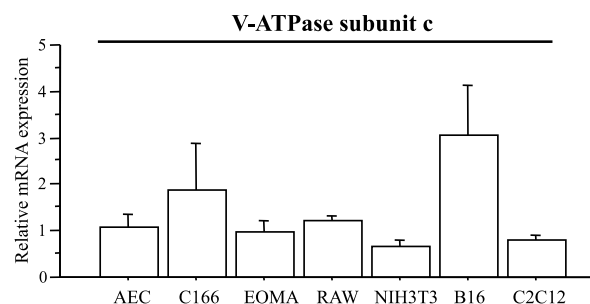
Figure 2. Expression of CA2 and V-ATPase in various types of cells. (A and B) Quantitative analysis for CA2 (A) or vacuolar H + -ATPase subunit c (B) mRNA expression in various cells. AEC, mouse aortic endothelial cells; C166, mouse endothelial cell line; EOMA, mouse endothelial cell line; RAW, mouse macrophage cell line; NIH3T3, mouse fibroblast cell line; B16, mouse melanoma cell line; C2C12, mouse myoblast cell line. Data are presented as mean \pm SE, n = 3 each.
