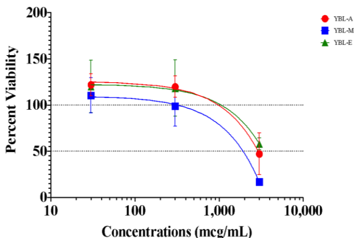
Fig. 1. Cytotoxicity of YB extracts in Vero cells.
