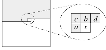
Fig. 1. The sample points of the fixed predictors.
