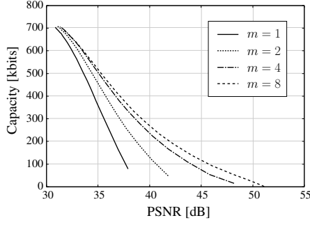
Fig. 3. The comparison of the performance for the number of element of the composed vector for an image “lena”.
