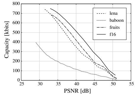
Fig. 6. The capacity of embedding information versus PSNR.
