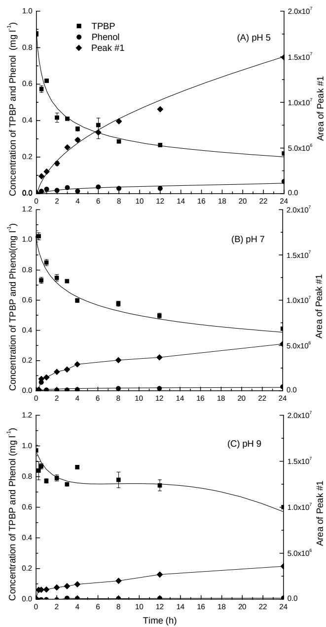
Fig. 2. Photodegradation of TPBP and the formation of phenol and the unknown Peak #1 in a sodium acetate buffer solution at: (A) pH = 5, (B) pH = 7, and (C) pH = 9.
