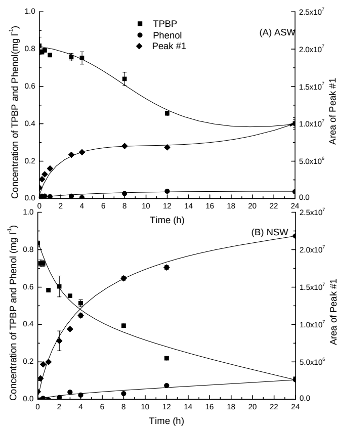
Fig. 3. Photodegradation of TPBP and the formation of phenol and the unknown Peak #1 in: (A) artificial seawater and (B) natural seawater.
