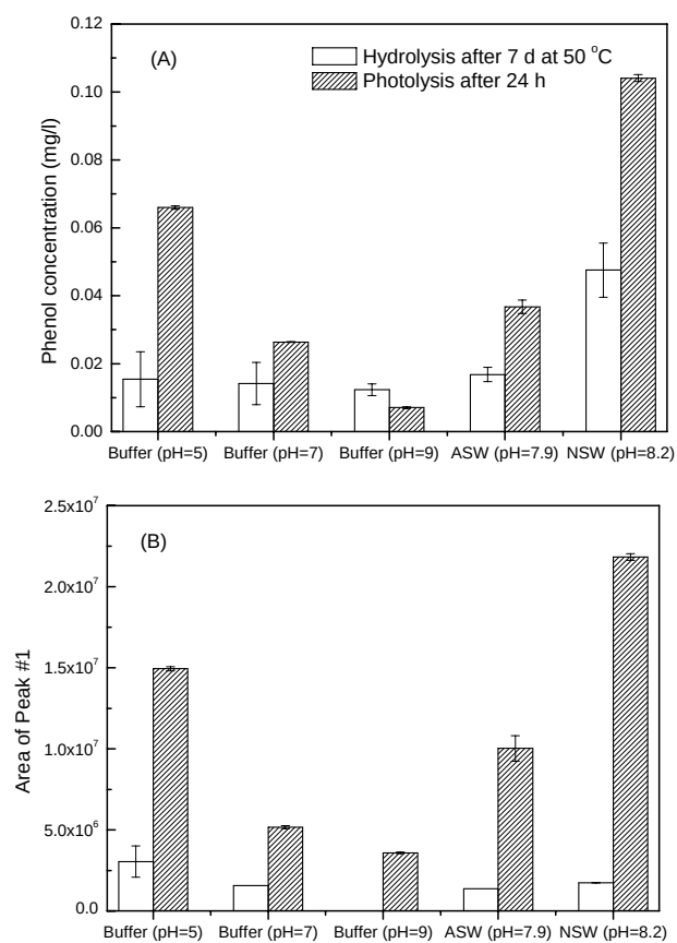
Fig. 5. Production of: (A) phenol and (B) unknown Peak #1 in the five aqueous solutions after hydrolysis and photolysis.
