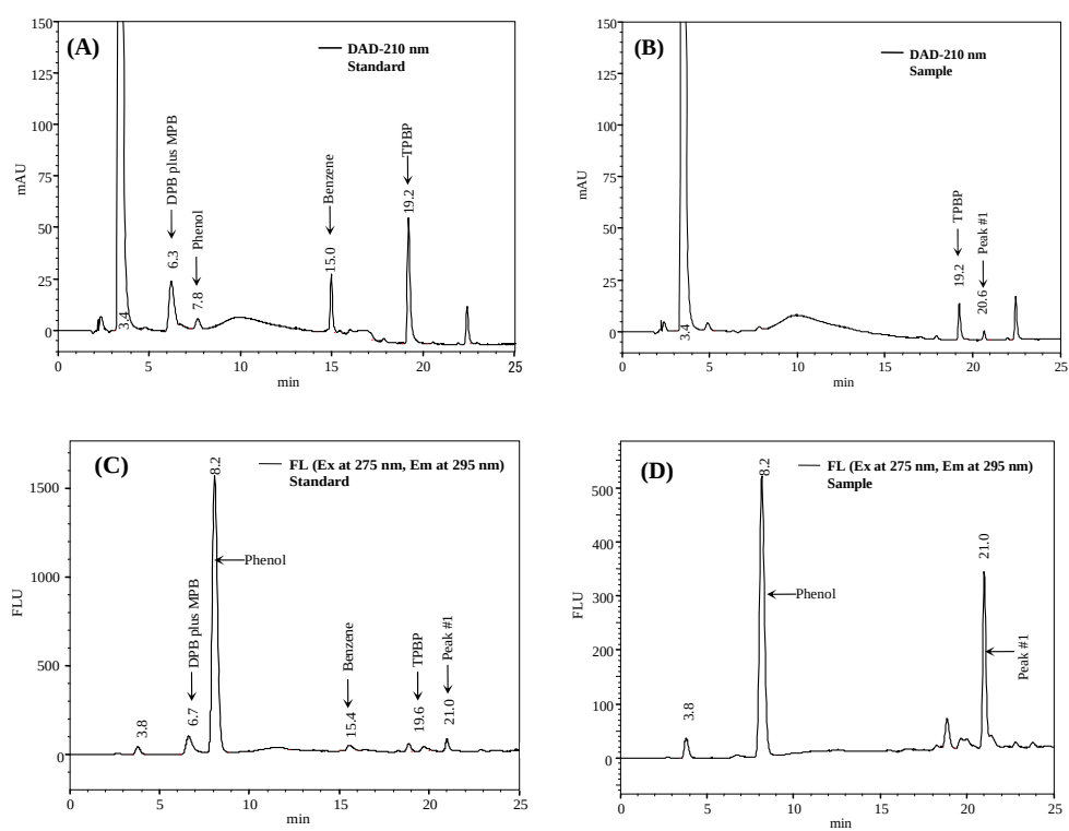
Fig. 1. HPLC chromatograms of a standard solution and a sample.
