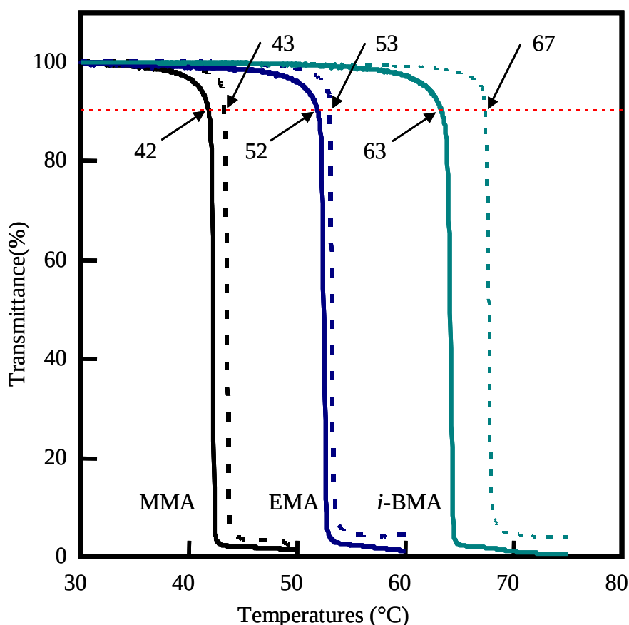
Fig. 4 Variations of transmittance of Emulgen 911 ( — ,14 mM ) and Emulgen 109P ( ..... ,17 mM ) aqueous solutions, in which MMA, EMA or i -BMA was saturated, as a function of temperature
