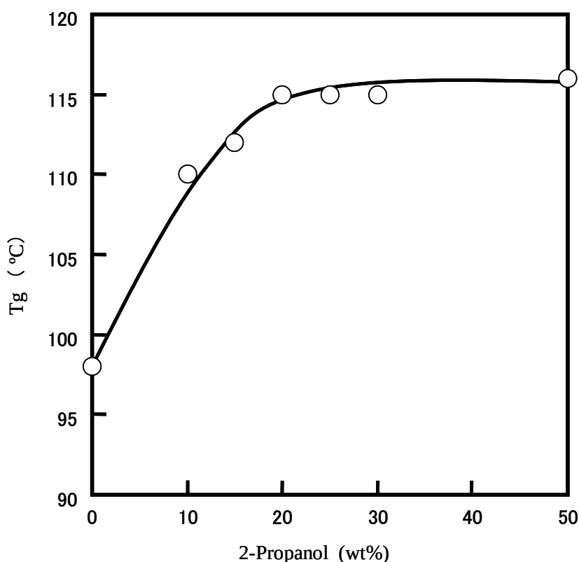
Fig. 2 Tg values of PMMA particles, which had been prepared by emulsifier-free emulsion polymerization and obtained from a mixture of the emulsifier free emulsion and the Emulgen 109P aqueous solution after washing with various compositions of 2-propanol aqueous solution
