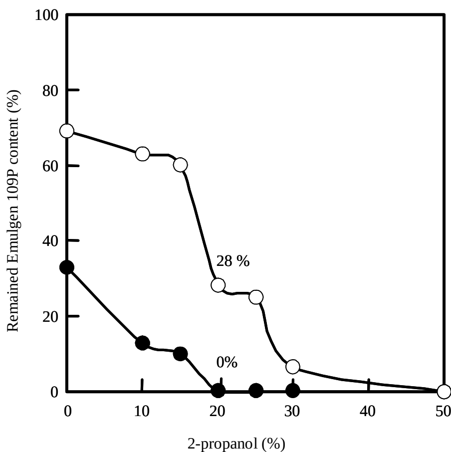
Fig. 1 Remained Emulgen 109P inside/on PMMA particles, which were prepared by emulsifier-present emulsion polymerization (○) and obtained from a mixture of Emulgen 109P and emulsifier-free PMMA particles (●), after washing with various compositions of 2-propanol aqueous solutions
