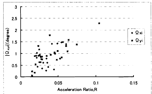
Fig.19 Estimate of impact angle and acceleration ratio
