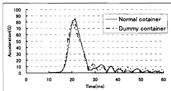
Fig.5 Comparison of composite acceleration on normal and dummy containers
