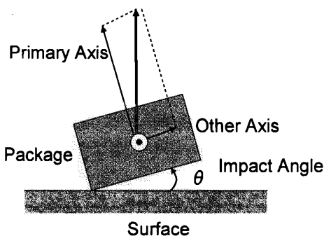
Fig.13 Image of relation between impact angle and other axis acceleration
