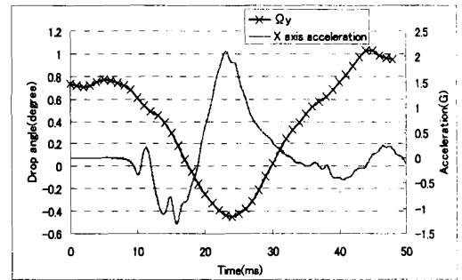
Fig.10 Time history of acceleration and drop angle
