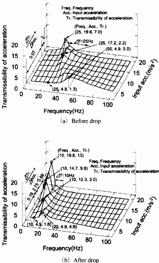
Fig. 8 Relation among input acceleration, frequency of input vibration and transmissibility of acceleration
