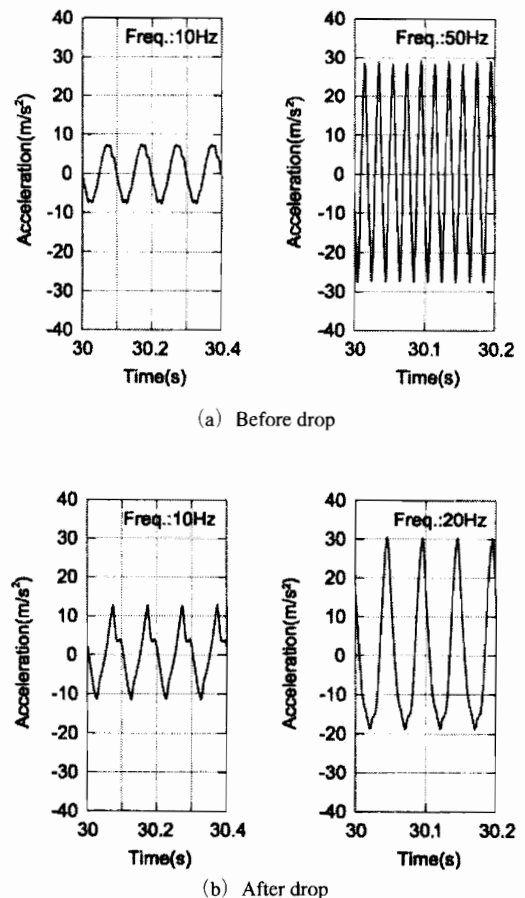
Fig. 9 Time history of acceleration of dummy (Input acceleration: 7.35 m/s 2 )
