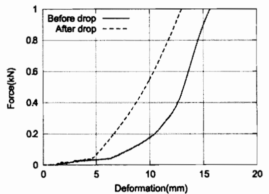
Fig. 3 Compression characteristics of corrugated cushioning materials before and after drop experiment
