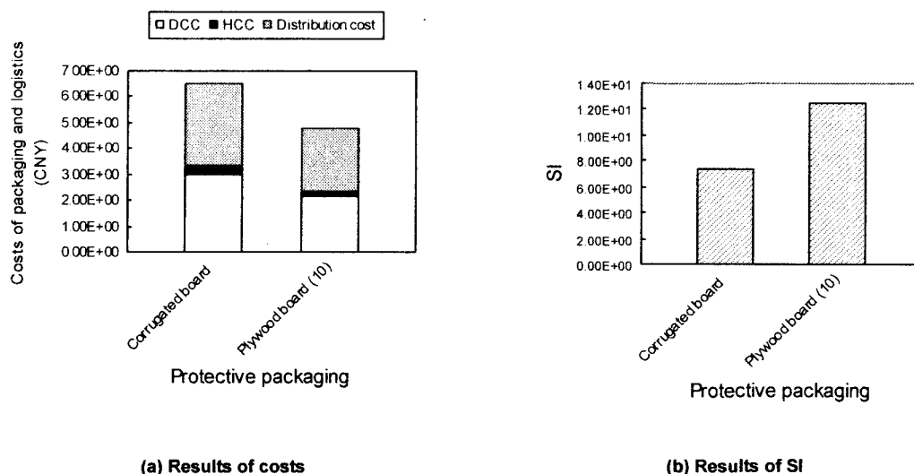
Fig. 4 Final results of the SA on the two protective packaging designs
