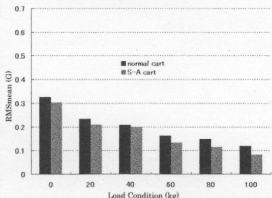
Fig.4 Comparison of Grms on Asphalt Road
