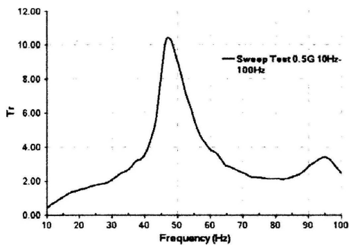
Fig.8 Frequency Response of Package
