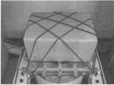
Fig.7 Vibration Test
