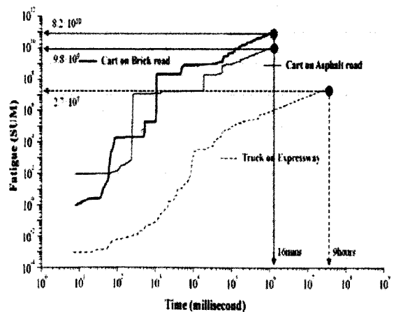
Fig.18 Cumulative Fatigue of Package on by Cart & Truck Distribution
