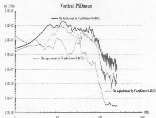
Fig.15 PSD of Dummy Package on Cart & Truck
