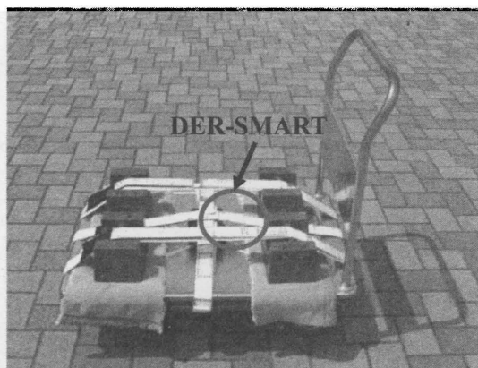
Fig.3 Shock-Absorbing Cart on Brick
