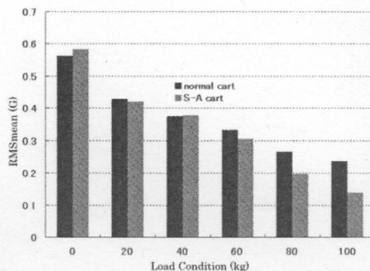
Fig.5 Comparison of Grms on Brick Road
