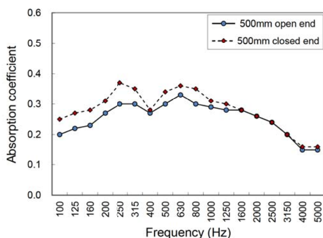
Figure 4. Measured results of the rectangular MPP space absorbers (RMSAs) of 500 mm x 500 mm square section. Solid line: open top ends; Dashed line: closed top ends with covers
