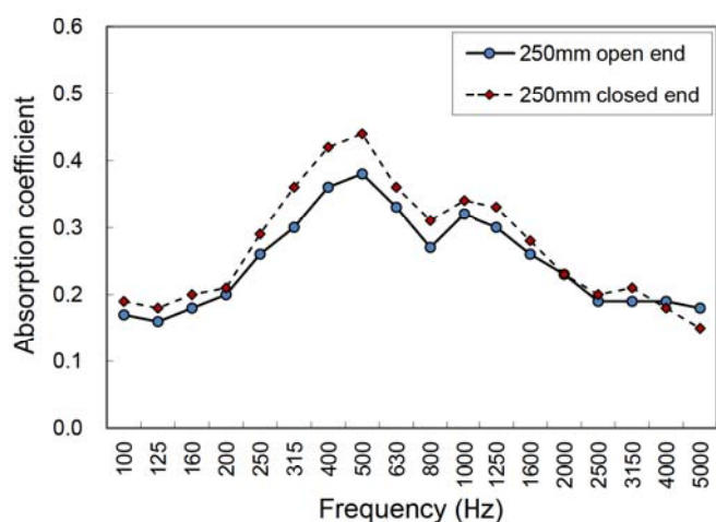
Figure 3. Measured results of the rectangular MPP space absorbers (RMSAs) of 250 mm x 250 mm square section. Solid line: open top ends; Dashed line: closed top ends with covers
