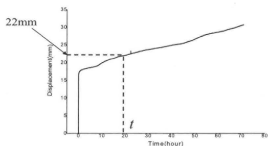
Fig.9 Time-series of Stacking Boxes Displacement
