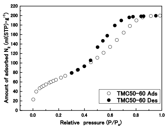
Fig.6 Adsorption-desorption isotherm of the hybrid membrane (TMC50-60); open symbols: adsorption, solid symbols: desorption
