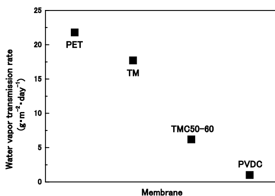
Fig.3 Water vapor transmission rates of the hybrid membranes (PET, TM, TMC50-60 and PVDC)
