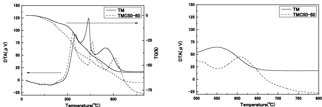
Fig.5 Thermal behaviors of the hybrid membranes (TM and TMC50-60) (A) TG/DTA curves between ambient temperature and 800°C (B) DTA curves between 500°C and 800°C
