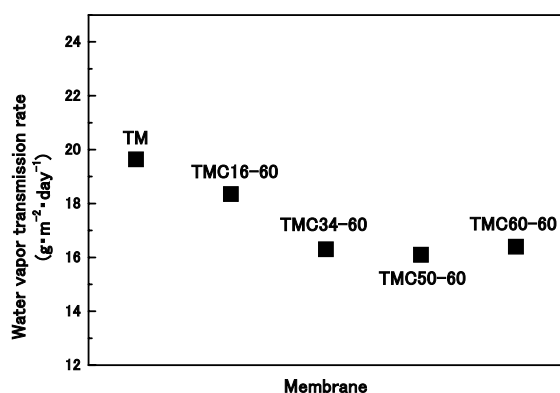
Fig.2 Water vapor transmission rates of the hybrid membranes (TM, TMC16-60, TMC34-60, TMC50-60 and TMC60-60)
