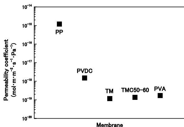
Fig.4 Oxygen Permeability coefficient of the hybrid membranes (PP, PVDC, TM, TMC50-60 and PVA)
