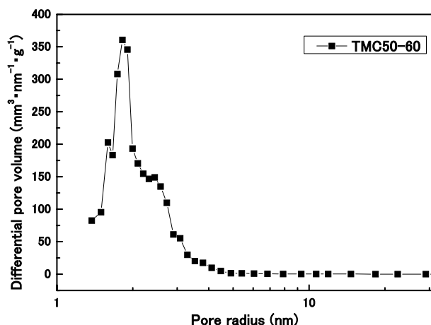
Fig.7 Pore size distribution of the hybrid membrane (TMC50-60)
