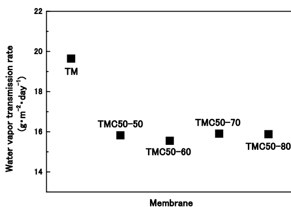
Fig.1 Water vapor transmission rates of the hybrid membranes(TM, TMC50-50, TMC50-60, TMC50-70 and TMC50-80)
