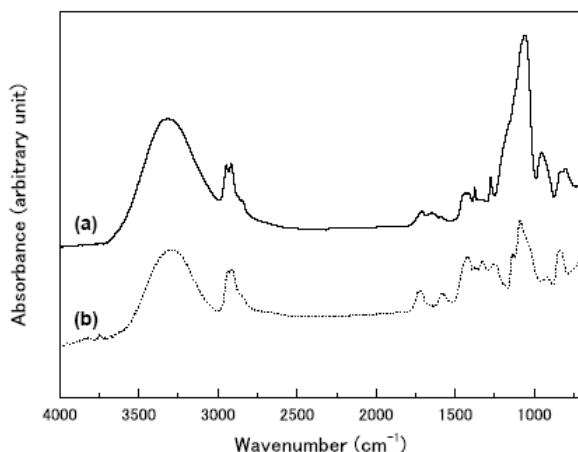
Fig. 4 IR spectra of (a)N40 and (b)T215.
