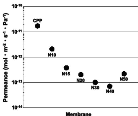
Fig. 6 Oxygen permeances through CPP and the hybrid films (N10, N15, N20, N30, N40 and N50).
