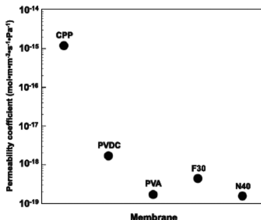
Fig. 7 Oxygen permeability coefficients of CPP, PVDC, PVA, F30 and N40.
