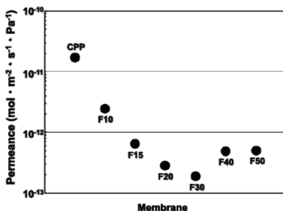
Fig. 5 Oxygen permeances through CPP and the hybrid films (F10, F15, F20, F30, F40 and F50).
