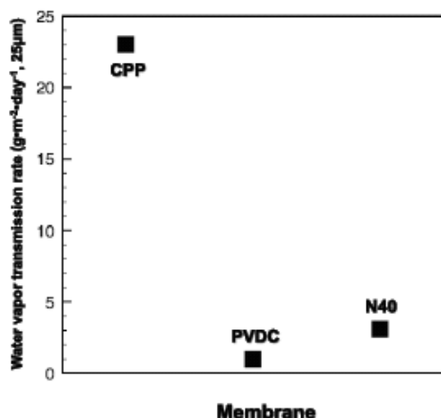
Fig. 8 Water vapor transmission rates of CPP, PVDC and N40.
