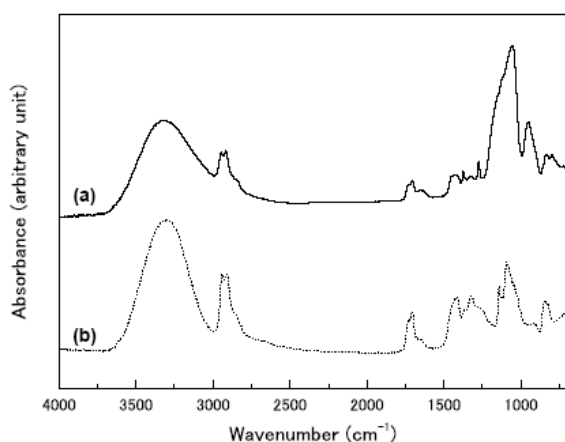
Fig. 3 IR spectra of (a)F30 and (b)Z100.
