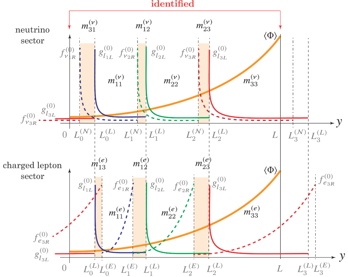
Figure 6. A schematic figure of the correspondence between the components of the mass matrices and the overlap integrals. The orange colored regions indicate the off-diagonal components of the mass matrices. m_{ij}^{(\nu)} corresponds to the overlap of g_{l_{iL}}^{(0)} , f_{\nu_{jR}}^{(0)} and m_{ij}^{(e)} corresponds to that of g_{l_{iL}}^{(0)} and f_{e_{jR}}^{(0)} .
