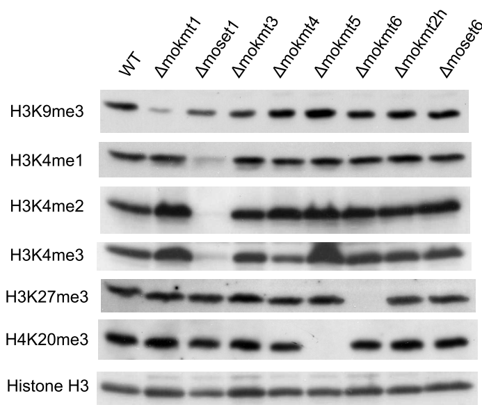
Fig 1. Western blotting analysis of histone modifications in KMT mutants. Total protein extracted from M. oryzae cells was subjected to 15% SDS polyacrylamide gel electrophoresis, and probed with antibodies against H3K4me1 (Active Motif #39298), H3K4me2 (Active Motif #39141), H3K4me3 (Active Motif #39159), H3K9me3 (Active Motif #39161), H4K20me3 (Active Motif #39181), and a C-terminal peptide of histone H3 (Active Motif #39163).
