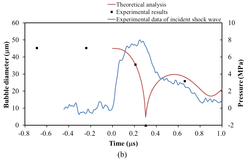
Fig. 7 Observation of the motion of a microbubble induced by interaction with an underwater shock wave: the initial bubble diameter is 45 \mu\text{m} . (a) Images of the interaction of a microbubble with an underwater shock wave as obtained by the SIM camera. (b) Comparison of the experimentally and analytically determined time variations of the bubble diameter
