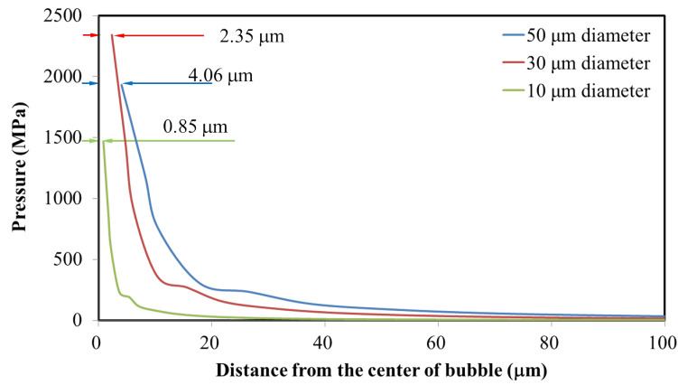
Fig. 4 Pressure attenuation of rebound shock waves generated by collapse motion of microbubbles of diameters 10, 30, and 50 \mu\text{m}
