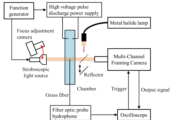
Fig. 6 Schematic diagram of the optical arrangement for visualizing the collapse motion of a microbubble using an ultra-high-speed framing camera
