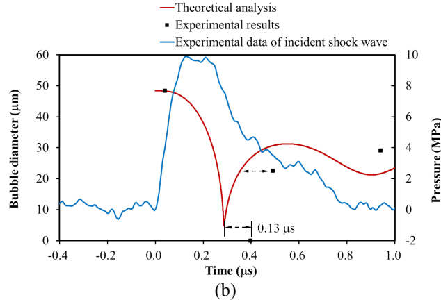
Fig. 9 Observation of microbubble motion induced by interaction with an underwater shock wave: the initial bubble diameter is 48.3 \mu\text{m} . (a) Images of the interaction of a microbubble with an underwater shock wave as obtained by the SIM camera. (b) Comparison of experimentally and analytically determined time variations of the bubble diameter
