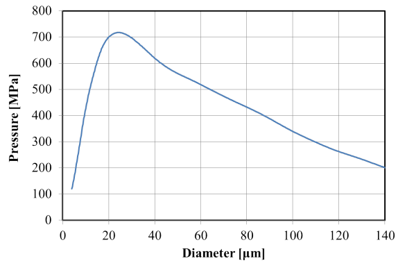
Fig. 3 Maximum internal pressure vs. initial bubble diameter
