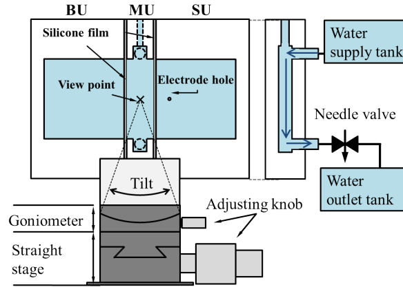
Fig. 5 Schematic diagram of the experimental water tank that comprises three components: the shock wave generation unit (SU), the microbubble position control unit (MU), and the buffer unit (BU).
