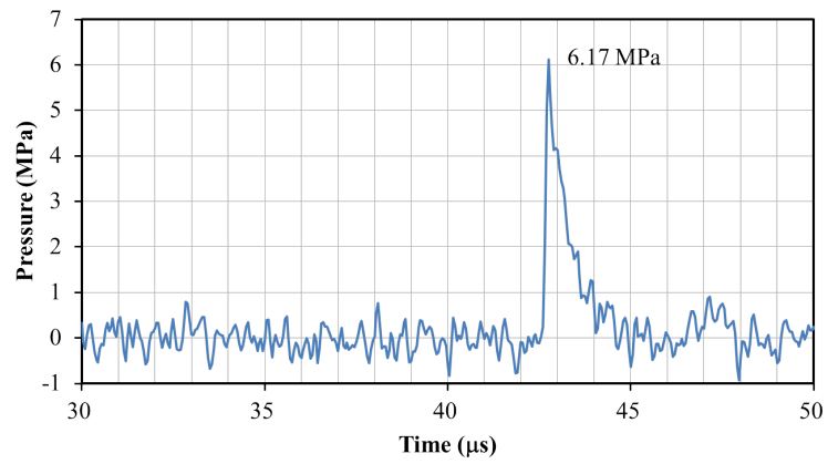
Fig. 1 Pressure profile of an experimental external spherical shock wave measured at 60 mm from the electrical discharge point
