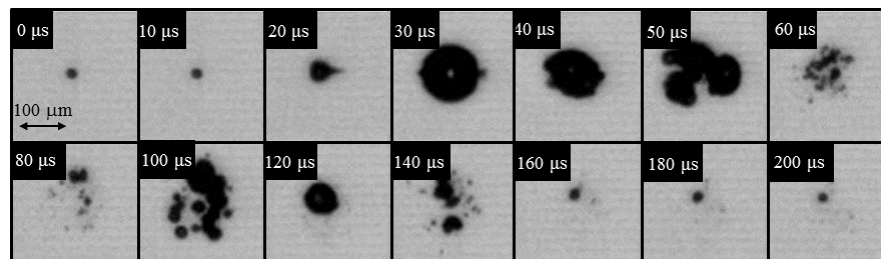
Fig. 12 Behavior of a single microbubble after the first rebound induced by an underwater shock wave
