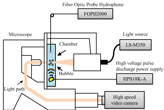
Fig. 11 Microscopic observation setup for the interaction of single and multiple microbubbles with an underwater shock wave
