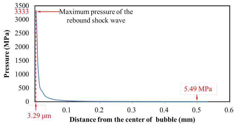
Fig. 8 Numerical analysis of the pressure attenuation of the experimental underwater shock wave due to the rebound shock wave for a microbubble of initial diameter 45 \mu\text{m} exposed to the shock wave
