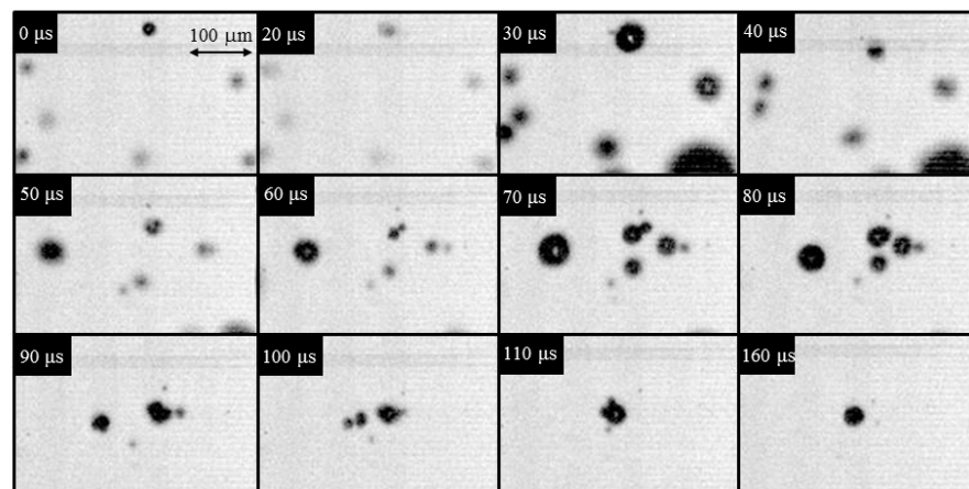
Fig. 13 Coalescent behavior of multiple microbubbles after their collapse induced by an underwater shock wave
