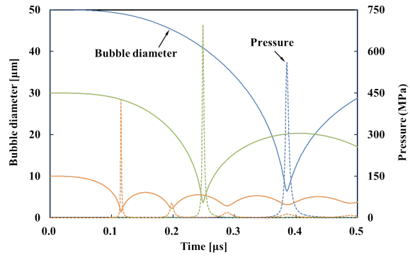
Fig. 2 Time variation of the bubble diameter and internal pressure
