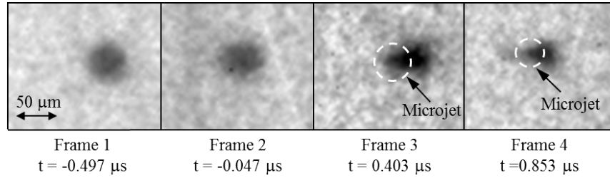
Fig. 10 Images of non-spherical collapse of microbubble induced by a shock wave: the initial bubble diameter is 48.3 \mu\text{m}
