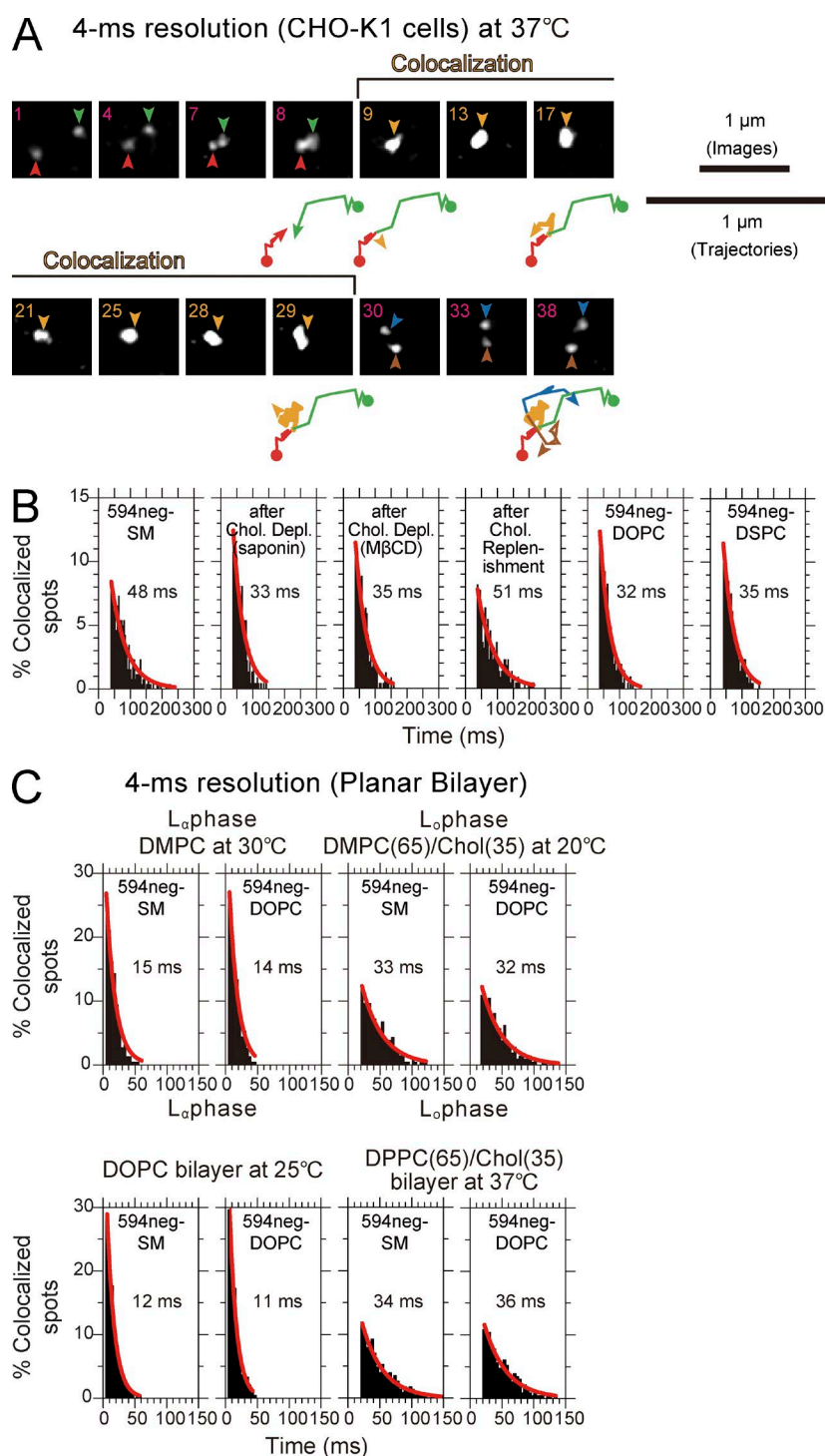
Figure 7. Transient ( \sim 15 -ms) molecular-scale colocalization of two 594neg-SM molecules at raft-related structures in the CHO-K1-cell PM at 37°C, recorded at a 4-ms resolution, which was undetectable in artificial lipid bilayers. (A) Typical image sequence of two diffusing 594neg-SM molecules (red and green arrowheads before colocalization; blue and brown arrowheads after colocalization and codiffusion (orange arrowheads). The number in the upper-left corner in each image indicates the number of frames. Trajectories are shown in a twofold magnified scale (displayed intermittently). The initial points of the trajectories are shown by closed circles. The end points of the trajectory shown by the arrowheads matched the fluorescent spots indicated by arrowheads in the image right above the trajectory. The green, red, orange, dark-blue, and brown colors indicate molecules (colors matched with those in the arrows in the images) before, during, and after colocalization, respectively. (B) Duration distributions for individual homo-colocalization events for single molecules of 594neg-SM (under various conditions), 594neg-DOPC, and 594neg-DSPC. All of the distributions could be fitted by single-exponential decay functions, but because the short molecular interaction lifetimes, the durations for incidental colocalization and those for colocalization including the molecular-scale interaction could not be separated. The decay time constants are shown in the boxes. The number of the observed colocalization events were 260, 223, 237, 220, 206, and 243 from left to right. (C) The duration distributions of individual homo-colocalization events for single 594neg-SM and 594neg-DOPC molecules in artificial planar bilayers in L_{\alpha} or L_{\beta} phase observed at a 4-ms time resolution, showing that the homo-colocalization of 594neg-SM, which was prolonged from that of 594neg-DOPC, in the cellular PM (48 vs. 33 ms), did not occur in either L_{\alpha} or L_{\beta} artificial planar lipid bilayers. For L_{\alpha} membranes, DMPC bilayers (30°C) and DOPC bilayers (25°C) were used, whereas for L_{\beta} membranes, DMPC-cholesterol (65:35 mol/mol; 20°C) and DPPC-cholesterol (65:35 mol/mol; 37°C) were used. The numbers of the observed colocalization events were 223, 225, 206, and 210 from left to right in the top row and 221, 243, 227, and 231 from left to right in the bottom row.
