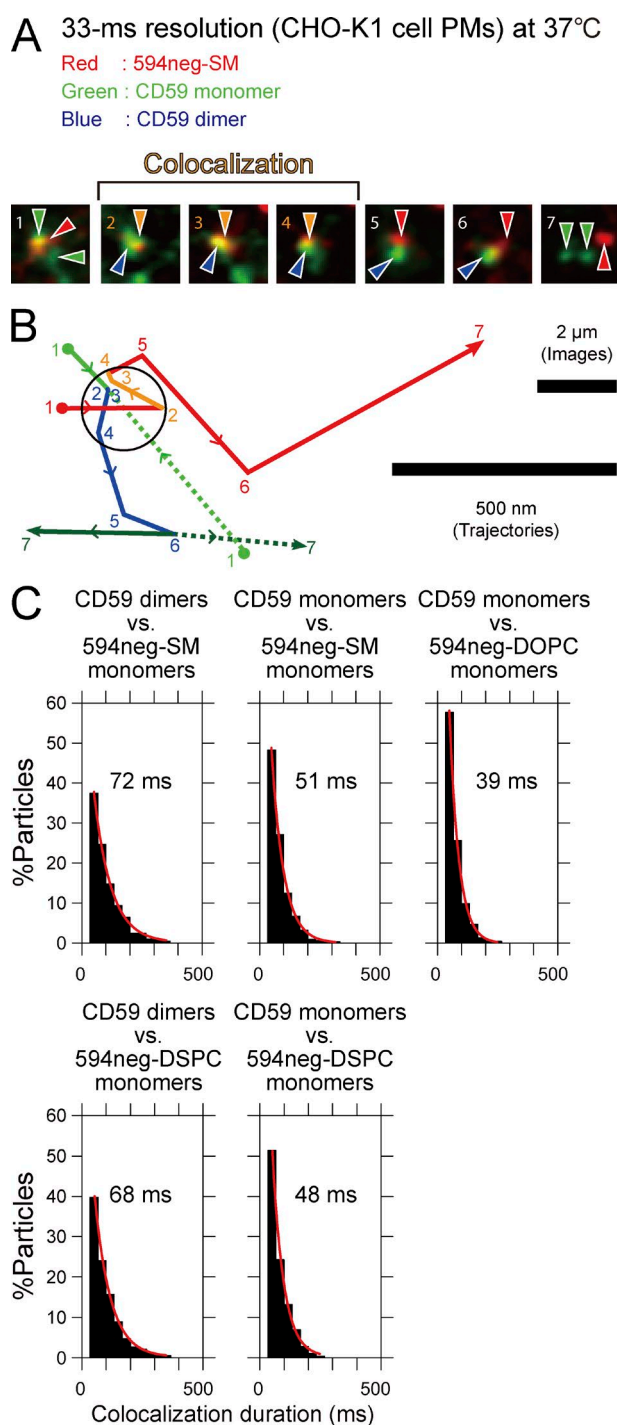
Figure 8. Single molecules of 594neg-SM were frequently and transiently recruited to CD59 monomers and CD59-homodimer rafts in quiescent cells for 12 and 33 ms, respectively. (A) Typical superimposed video frame sequences of a 594neg-SM molecule (red spot) and two CD59 molecules (green spots) in the CHO-K1-cell PM, observed at a 33-ms resolution. Two individual CD59 monomers formed a dimer and diffused together (distances \leq 240 nm) for the period of four video frames (between frame 2 and frame 6), and simultaneously, these CD59 molecules became colocalized with a 594neg-SM molecule between frame 2 and frame 4. (B) Trajectories of the molecules shown in A. The positions of individual molecules in each image frame shown in A are indicated by the frame numbers. Color coding: 594neg-SM in red (orange during colocalization with CD59); CD59 monomers in green solid and dotted lines, and homo-colocalized CD59 molecules (CD59 homodimer raft) in blue. Colocalization of 594neg-SM and CD59 is shown in the circle, with a 240-nm diameter (see Online
