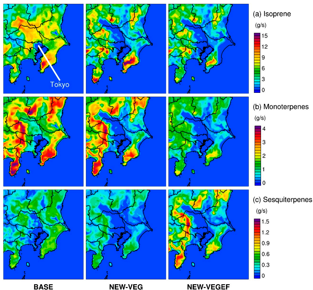
Figure 5. Horizontal distributions showing mean emission rates of (a) isoprene; (b) monoterpenes, and (c) sesquiterpenes estimated in BASE, NEW-VEG, and NEW-VEGEF cases during the target period in d04.
