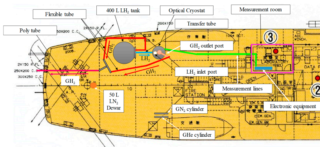
Figure 5. Setup of the experimental apparatus.
