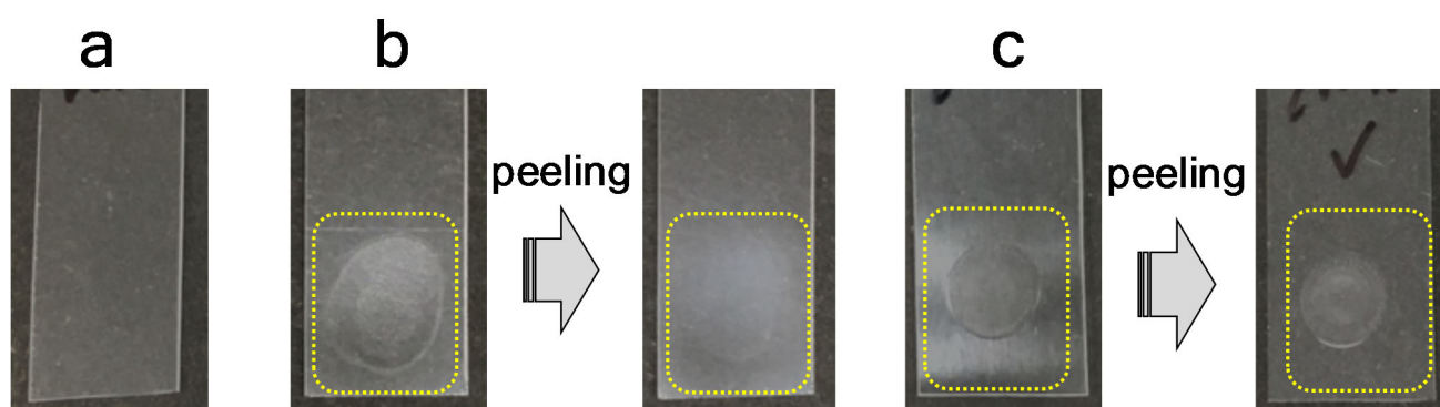
Figure 2. Optical images of scotch-tape peeling tests for PP substrates. (a) Bare PP, (b) PP drop-cast with a PMFP solution, and (c) PP drop-cast with a MPO/PMFP solution. Polymer solution (3 \mu\text{L} ) was drop-cast on the PP substrate (coating diameter was \sim 5 mm) and dried under vacuum overnight.
