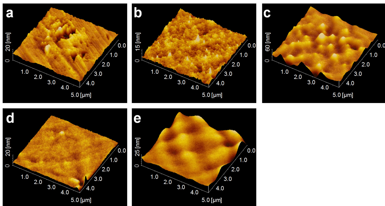
Figure S9. AFM images of PP surfaces dip-coated with various polymers (5 \mu\text{m} \times 5 \mu\text{m} ). (a) Bare PP, (b) surface dip-coated with MPO, (c) surface dip-coated with MPO/poly(MMA- r -PEGMA), (d) surface dip-coated with MPO/poly(MMA- r -PFEA8), and (e) surface dip-coated with MPO/PMFP.
