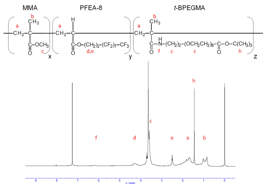
Figure S5. ^1\text{H-NMR} spectra of poly(MMA/PFEA8/ t -BPEGMA) (PMFB).
