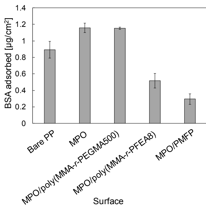
Figure 6. Amount of BSA adsorbed on bare and dip-coated PP surfaces.
