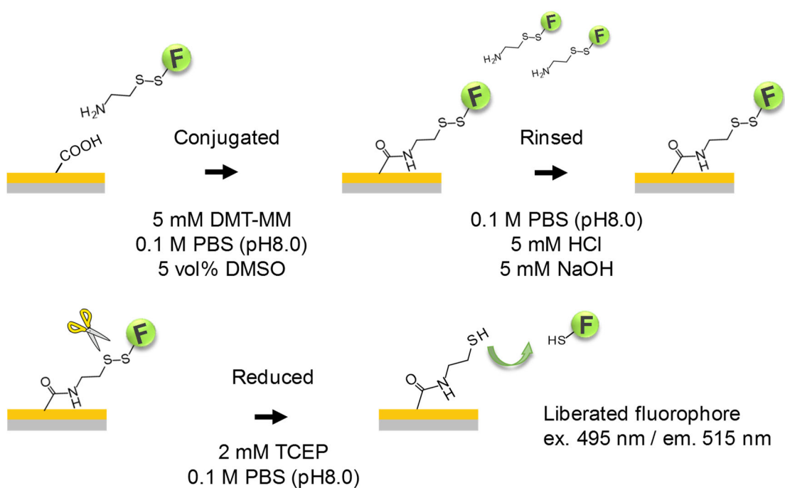
Figure S7. Schematic illustration of the quantification of carboxylic groups on a solid surface using cleavable fluorescent compounds.
