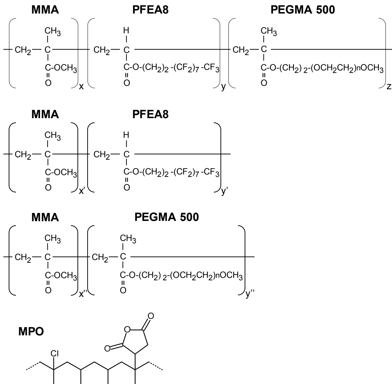
Figure 1. Chemical structures of a terpolymer containing perfluoroalkyl (Rf)-conjugated monomers and poly(ethylene glycol) monomers (PMFP), poly(MMA-r-PFEA8), poly(MMA-r-PEGMA500) and modified polyolefin (MPO).
