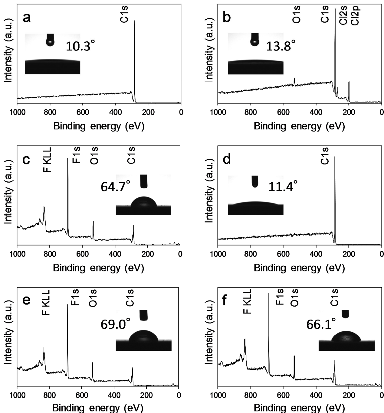
Figure 3. XPS spectra of bare and dip-coated PP surfaces. Insets are optical images of oil-contact-angle measurements. (a) Bare PP, (b) PP dip-coated with MPO after the peeling test, (c) PP dip-coated with PMFP before the peeling test, (d) PP dip-coated with PMFP after the peeling test, (e) PP dip-coated with MPO/PMFP before the peeling test, and (f) PP dip-coated with MPO/PMFP after the peeling test.
