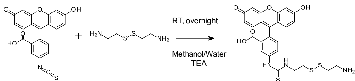
Figure S6. Synthesis of a cleavable fluorescent compound.
