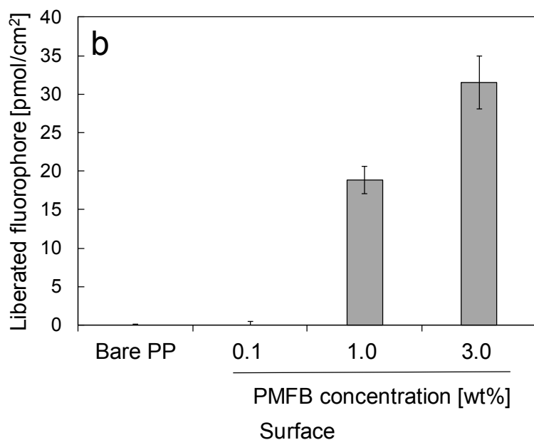
Figure 8. Surface density of carboxy groups on PP surfaces dip-coated with a mixture solution of MPO/PMFB. a) Effect of MPO concentration (PMFB concentration was 1.0 wt%). b) Effect of PMFB concentration (MPO concentration was 1.0 wt%).
