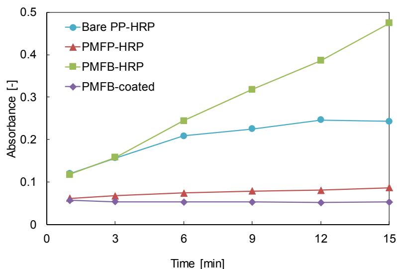
Figure S10. Time courses of the oxidation of 2,2'-azino-bis(3-ethylbenzothiazoline-6-sulphonic acid) (ABTS) catalyzed by HRP immobilized on surfaces. Bare PP- HRP, PMFP-HRP and PMFB-HRP were PP substrates that underwent the HRP-immobilization procedure using a condensation agent. PMFB-coated means a PMFB-coated PP substrate without HRP immobilization.
