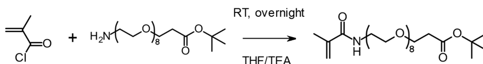
Figure S4. Synthesis of t -BPEGMA monomer.
