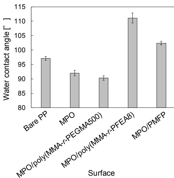
Figure 5 Water contact-angle measurements for bare and dip-coated PP surfaces.
