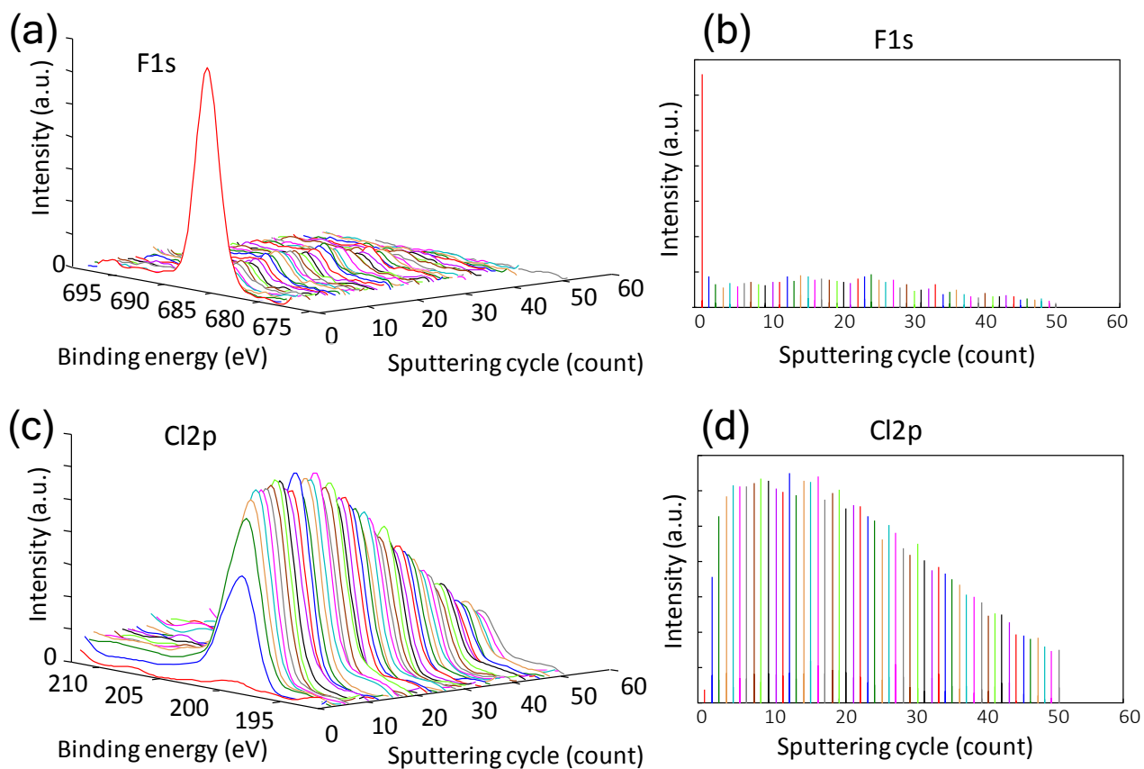
Figure 4 XPS depth profiles of a PP surface dip-coated with MPO/PMFP. (a and b) F 1s and (c and d) Cl 2p . Atomic intensities were shown as a function of sputtering cycle.
