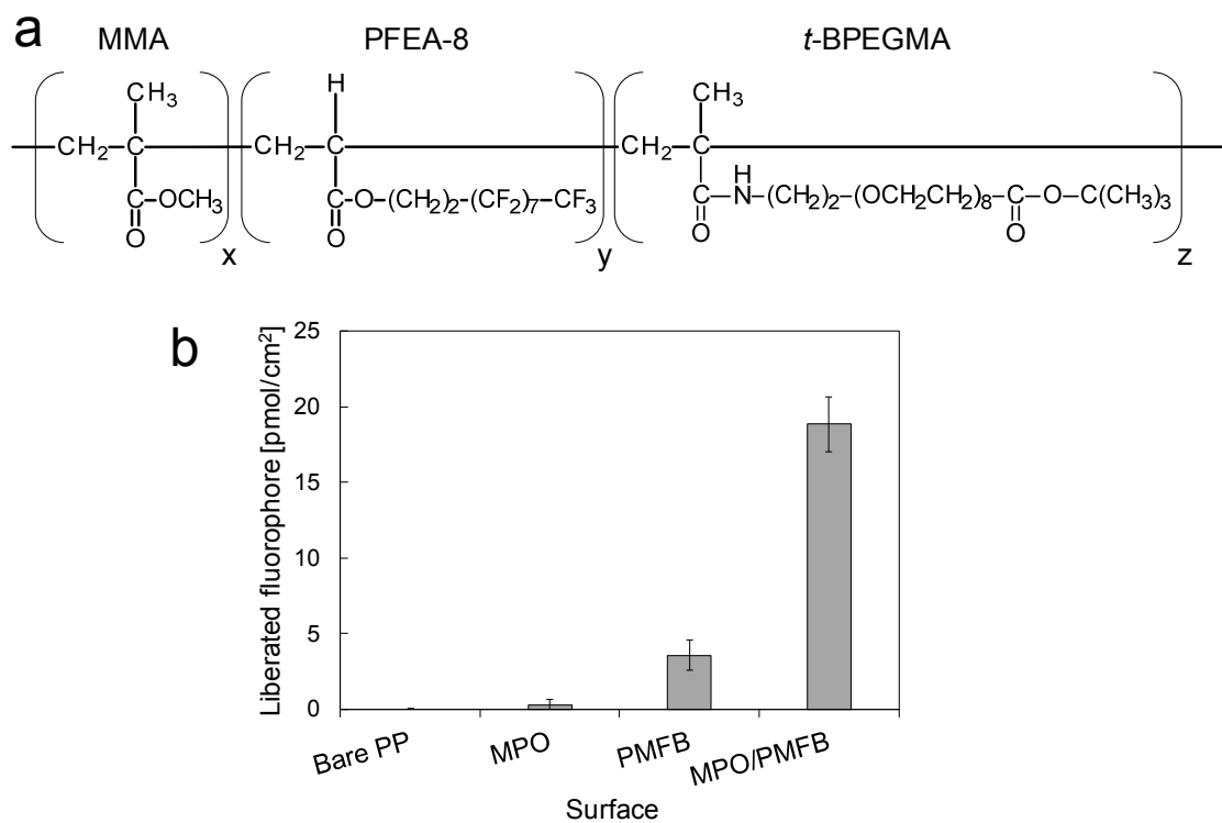
Figure 7. a) Chemical structure of poly(MMA- r -PFEA8- r - t -BPEGMA) (PMFB). b) Surface density of carboxy groups on PP dip-coated with various polymers. Each polymer was used at 1.0 wt% in toluene.
