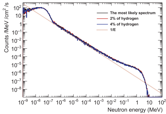
Fig. 8. The most likely spectrum (sample 1 with 3% of h.e.) of ambient neutrons produced by (\alpha, n) reactions and spontaneous fission in Lab-B at the Kamioka Observatory.
