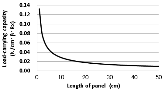
Fig.3 Graph of load-carrying capacity of panel
