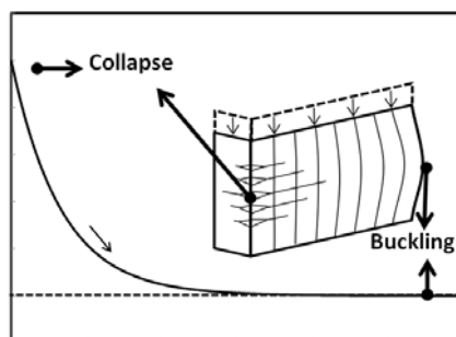
Fig.11 Feature of load-carrying capacity of panel
