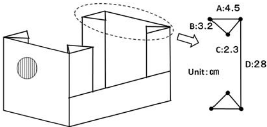
Fig.9 Design of newly developed box
