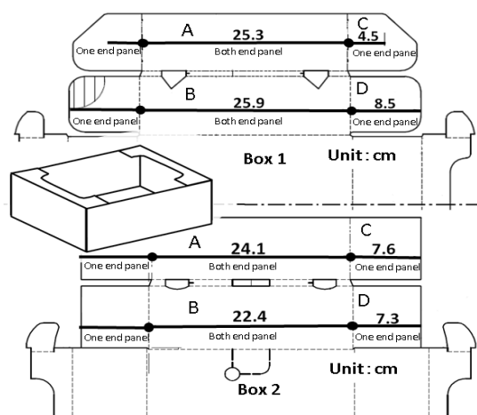
Fig.8 Developments of folder type boxes
