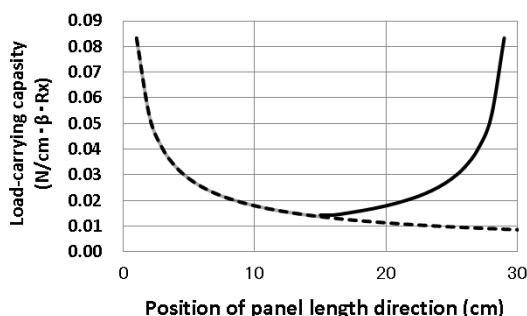
Fig.5 Distribution of load-carrying capacity along the direction of length Solid line shows feature of equation-5 Dashed line shows feature of equation-4
