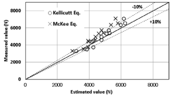
Fig.7 Correlation between estimated and measured value
