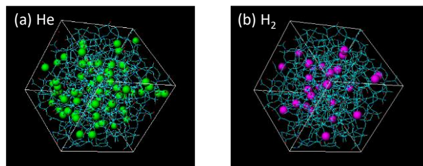
Figure 7. Snapshot of the distribution of sorption sites for probing: (a) helium and (b) hydrogen.
