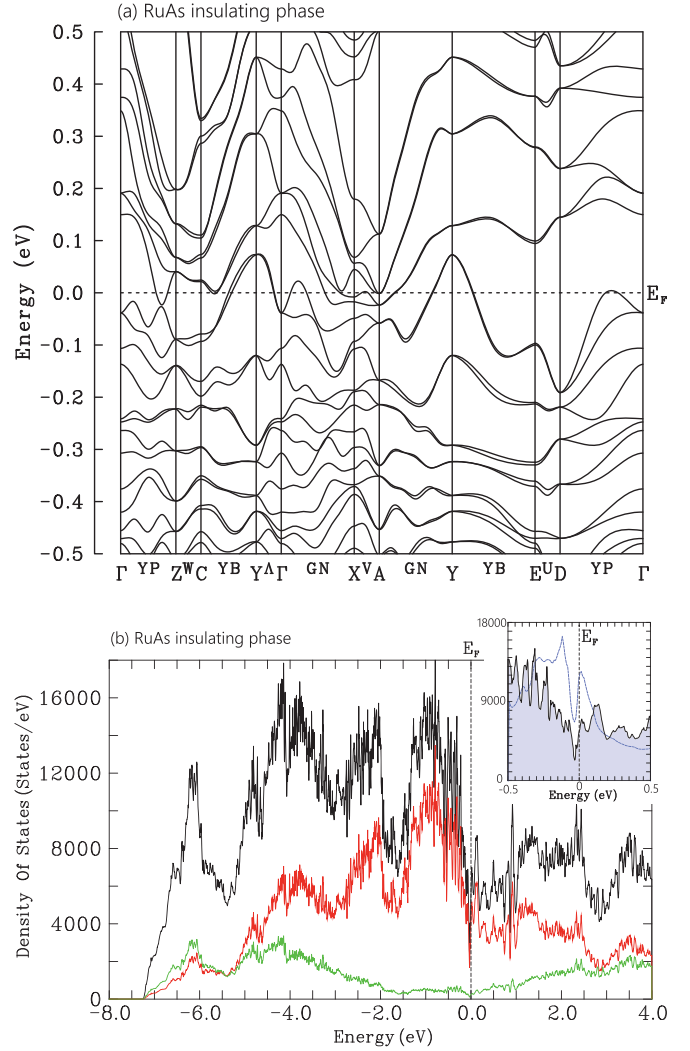
FIG. 9. The calculated energy dispersion in the vicinity of E_F and the DOS of RuAs in the insulating phase in the monoclinic P2_1/c space group. A gaplike feature is likely to appear in the DOS near E_F . In the lower panel, the black curve indicates the total DOS integrated in the whole k space. The red and green curves indicate the partial DOS originating from the Ru- 4d and As- 4p orbitals, respectively. In the inset, the solid line with the hatched region indicates the total DOS for the insulating state, while the dotted line shows the metallic state. Here, the DOS of the metallic phase is multiplied by 9 to adjust the difference in the size of the unit cell.
