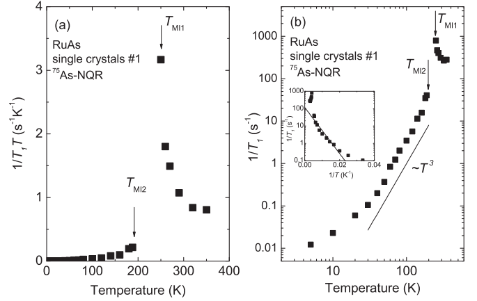
FIG. 6. Temperature dependence of (a) 1/T_1T and (b) 1/T_1 for RuAs. RuAs undergoes the insulating state accompanied by a strong development of some fluctuations. The T^3 behavior below T_{\text{MI2}} indicates that the energy gap of RuAs is anisotropic.
