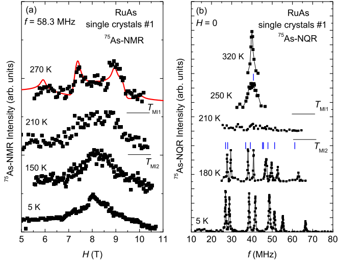
FIG. 5. (a) Field-swept NMR spectrum for RuAs measured at around 8 T. (b) NQR spectrum for RuAs measured at zero field. In the metallic state above T_{\text{MI1}} , the NMR spectrum obtained using many pieces of single crystals shows a typical powder pattern by assuming the unique As site, as shown by the red curve. This is consistent with the NQR spectrum observed at around 40.0 MHz. Below T_{\text{MI1}} , the broadened NMR spectrum and the suppression of the NQR intensity indicate the strong distribution of \nu_Q and \eta . In the ground state below T_{\text{MI2}} , several peaks are observed at the NQR measurement, indicative of the formation of the superlattice. The blue lines indicate the resonance frequencies calculated using the structural parameters at 293 K and 170 K.
