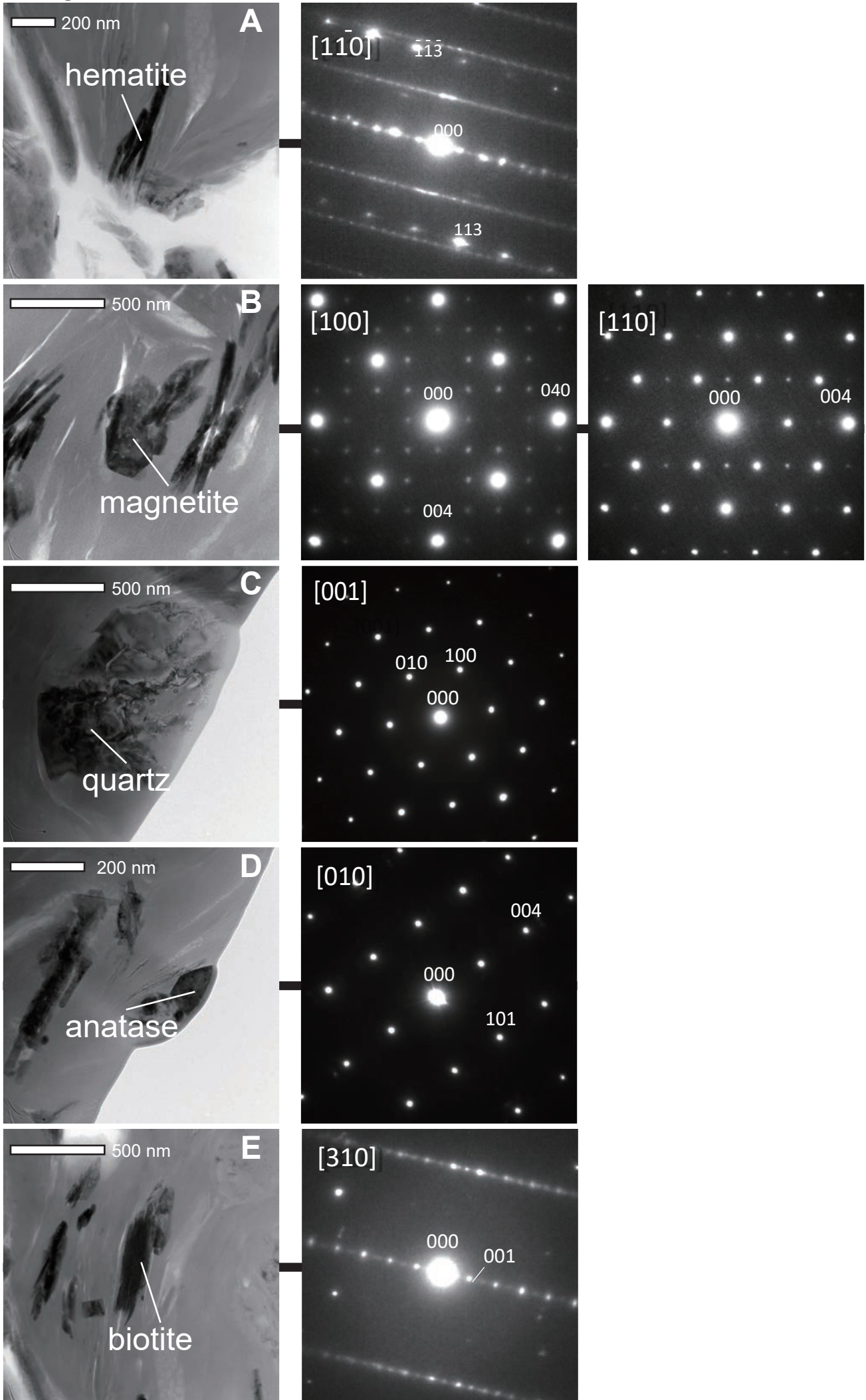
Figure R4. Bright field (BF) transmission electron microscopy (TEM) images and electron diffraction patterns for discrete particles of the D2 paleosol LS8 (magnetic extracts). (A) Hematite. (B) Magnetite. (C) Quartz. (D) Anatase. (E) Biotite.
