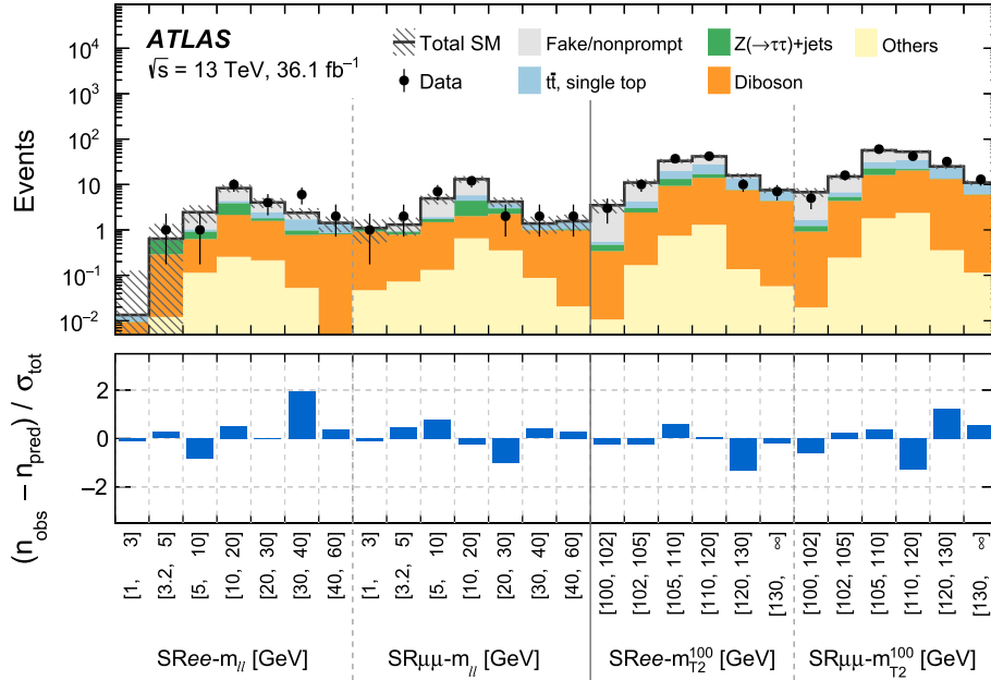
FIG. 9. Comparison of observed and expected event yields after the exclusion fit with the signal strength parameter set to zero in the exclusive signal regions. Background processes containing fewer than two prompt leptons are categorized as “Fake/nonprompt.” The category “Others” contains rare backgrounds from triboson, Higgs boson, and the remaining top-quark production processes listed in Table I. Uncertainties in the background estimates include both the statistical and systematic uncertainties, where \sigma_{\text{tot}} denotes the total uncertainty.
