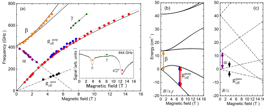
Fig. 3 (a) Electromagnetic-wave frequency versus resonance field derived from the observed EPR spectra, together with simulated curves, taking into account the ZFS parameters. Assignment of the branches is given in the text. The inset shows the magnified EPR data for 644 GHz, in which an additional weak absorption (the \gamma branch) was observed. (b) The calculated energy levels of hemin for B \parallel x, y , and vertical arrows indicate the corresponding EPR transitions for the field-swept data at 441 GHz. Curves for B \parallel x and y are almost overlapped and cannot be resolved in this scale. (c) The calculated energy levels of hemin for B \parallel z . Purple ( \alpha ) and black ( g_{\text{eff}}^{\text{para}} ) arrows indicate the corresponding EPR transitions for the field-swept data at 363 and 105 GHz, respectively.
