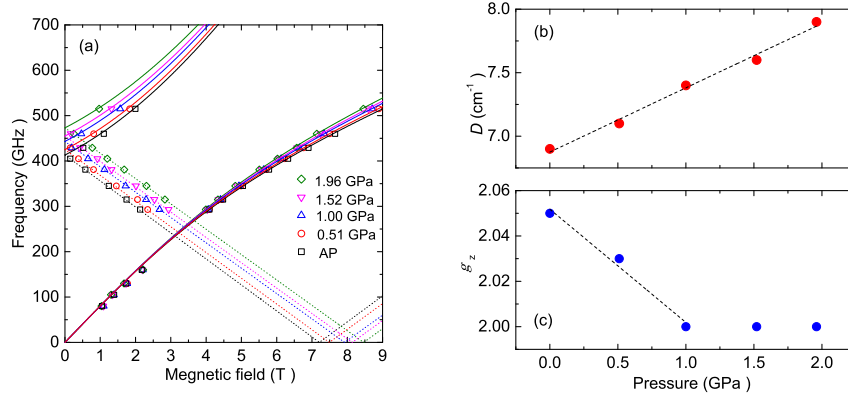
Fig. 5 (a) Electromagnetic-field frequency-resonance field diagram for all pressure values. Simulation curves (solid and dotted lines) are shown together. The pressure dependences of (b) D and (c) the intrinsic g_z are shown. Dotted straight lines are the fit result to the respective data.
