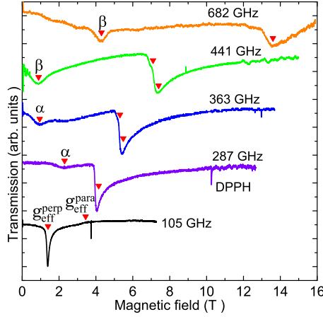
Fig. 2 Raw data of HFEPR spectra of hemin at selected frequencies. Spike-like signals near 4 and 10 T for 105 and 287 GHz, respectively, are attributed to the EPR signal of DPPH. Solid triangles indicate characteristic positions of the observed HFEPR signals.
