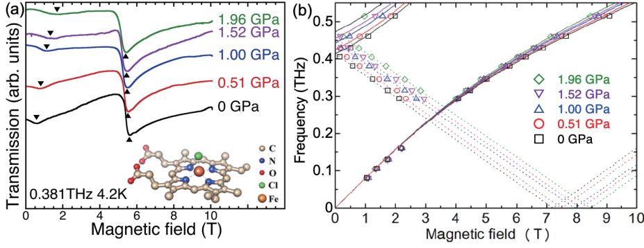
Fig. 5 (color online) (a) Pressure dependence of powder ESR spectra obtained at 0.381 THz and 4.2 K for hemin. (b) Frequency-field diagram at 4.2 K obtained at various pressures for hemin, made by modifying Fig. 4 in ref. [41].
