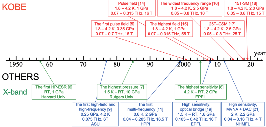
Fig. 1 (color online) History of high-pressure ESR. The upper row is our contribution; the lower row is the contribution by other groups. In the lower row, the line labeled “X-band” shows representative high-pressure X-band ESR systems. ASU and HPPI indicate Academy of Sciences of the Ukraine SSR (present-day National Academy of Sciences of Ukraine) and Institute for High Pressure Physics, respectively. See text for details.
