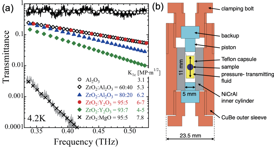
Fig. 2 (color online) (a) Frequency dependence of the transmittance of various ceramics. The K_{1c} value, which indicates fracture toughness, is also shown. The transmittance was measured at 4.2 K for a test piece with the same shape (12 mm × 30 mm). Because obtained data can be fitted almost linearly in a semi-logarithmic plot, only fitting results are shown except for the highest and lowest results. (b) Cross section of a hybrid-type pressure cell.
