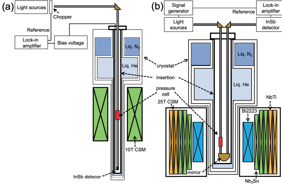
Fig. 3 (color online) Schematic diagram of high-pressure ESR systems using 10T-CSM (a) and 25T-CSM (b).
