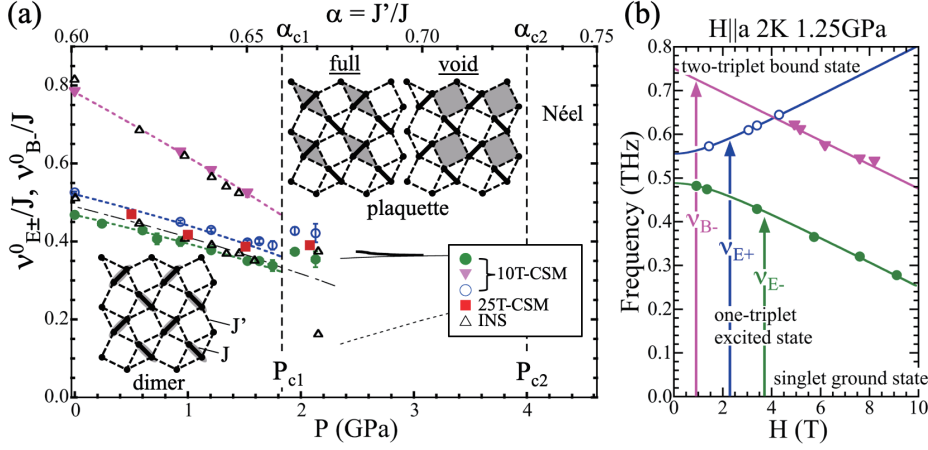
Fig. 4 (color online) (a) Pressure and interaction ratio \alpha = J'/J dependence of the excitation energy normalized J obtained by the 10T-CSM system for \text{SrCu}_2(\text{BO}_3)_2 , made by modifying Fig. 3 (b) in ref. [28]. The excitation energies obtained by the 25T-CSM system [17] and INS [33] are also plotted. Illustrations indicated by “dimer” and “plaquette” represent the singlet state formed by the spins in the shaded area. For the plaquette singlet state, there is a “full type”, which includes the diagonal interaction J , and a “void type”, which does not. (b) Frequency-field diagram for H \parallel a obtained at 2 K and 1.25 GPa, made by modifying Fig. 1 (b) in ref. [28]. The solid curves for \nu_{E\pm} are the fitting result by theoretical curves [38]. The solid line for \nu_{B-} is the linear fitting result.
