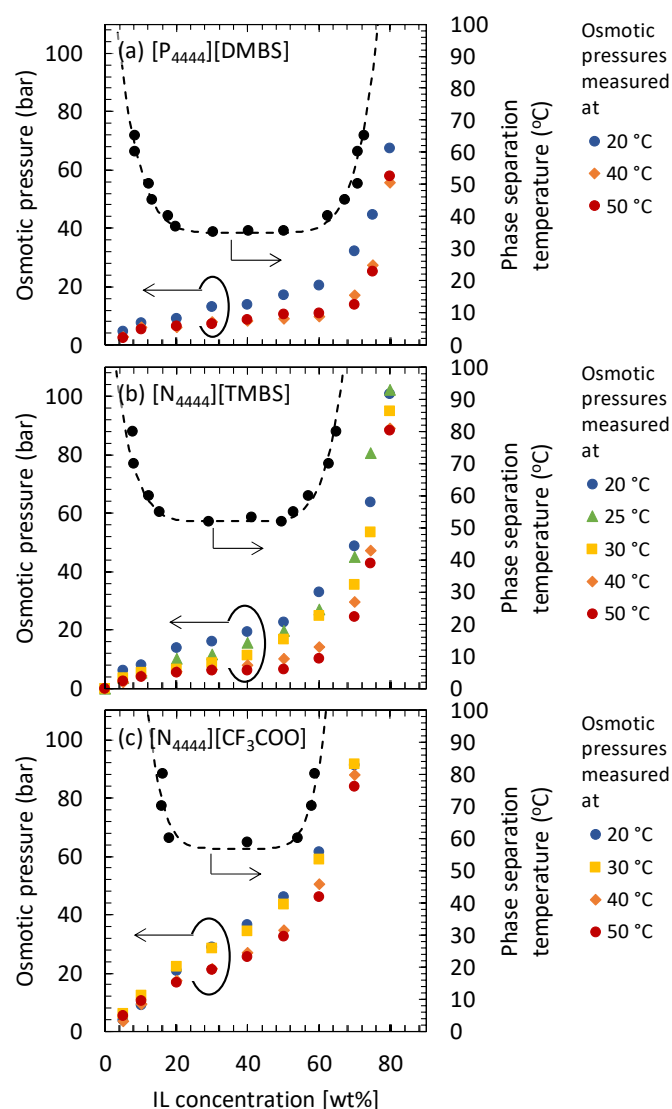
Figure 3. Phase diagram and temperature dependency of the osmotic pressure of thermo-responsive DS at different temperatures. (a) [P_{4444}][DMBS] , (b) [N_{4444}][TMBS] , and (c) [N_{4444}][CF_3COO] . The data other than the osmotic pressure of [N_{4444}][TMBS] aqueous solution measured at 25 °C were those previously reported in Ref. [32]. Reproduced with permission from Ref. [32]. Elsevier, 2021.
